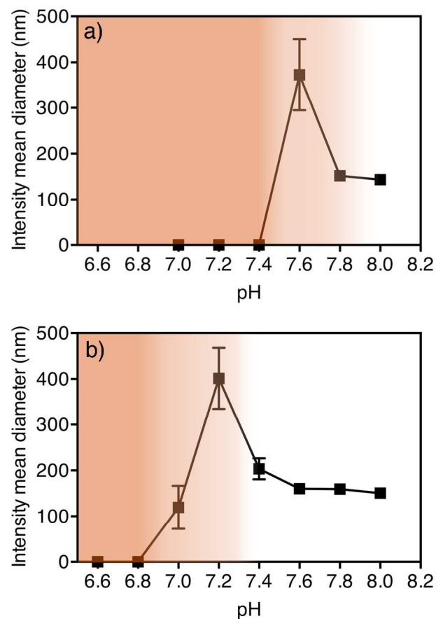
Figure 2. pH dissociation profiles of PDEAEMA dual component nanoparticles at a) 25 °C and b) 37 °C. The white unshaded region indicates nanoparticle stability whereas the dark shaded region indicates disassembled particles. The shaded gradient from light to dark indicates a region of nanoparticle instability.
