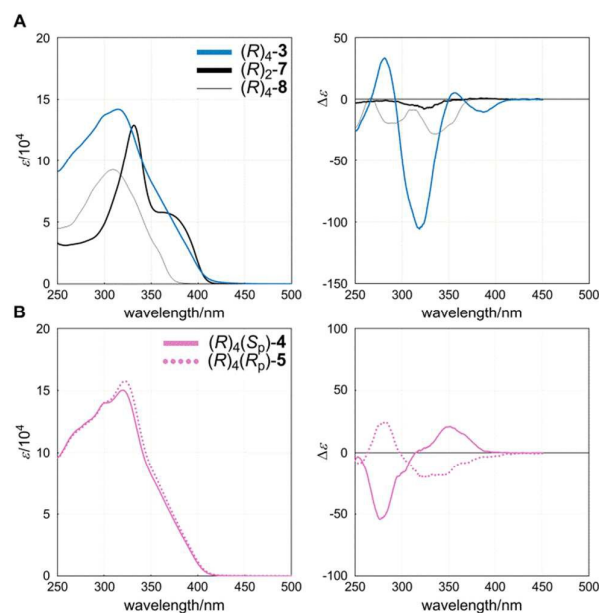
Fig. 4 UV (left) and CD (right) spectra of (A) ( R ) 4 - 3 , ( R ) 2 - 7 and ( R ) 4 - 8 , and (B) ( R ) 4 ( S p )- 4 and ( R ) 4 ( R p )- 5 . All spectra were measured in dichloromethane at room temperature.
