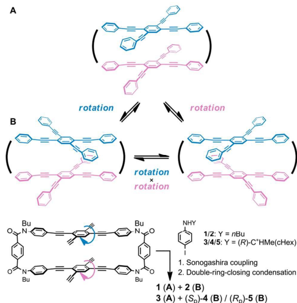
Scheme 2 The "obverse and/or reverse" relation in two cyclophanes A and B , and a synthetic strategy for obtaining both quadruply-bridged cyclophanes A and B .
