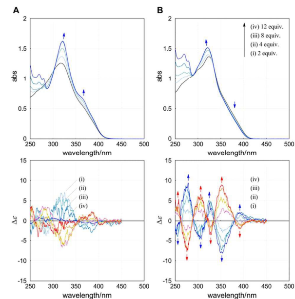
Fig. 6 UV (upper) and CD (lower) spectra of 1 (A) ( 7.5 \times 10^{-5} M) and 2 (B) ( 9.9 \times 10^{-5} M) in the presence of ( R ) 2 - 6 (blue lines) or ( S ) 2 - 6 (red lines) [0 (black, host only), 2, 4, 8 and 12 equiv.]. All spectra were measured in dichloromethane at 293 K.
