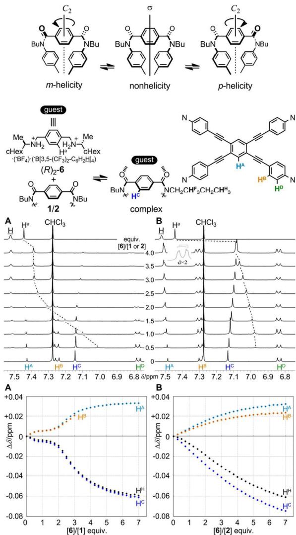
Fig. 5 Partial 1 H NMR (400 MHz) spectra of 1 ( A ) (0.5 mM) in the presence of ( R ) 2 - 6 [0 (host only)-4 equiv.] and the spectrum of ( R ) 2 - 6 (top), and titration curves for the complexation of 1 ( A )/ 2 ( B ) with ( R ) 2 - 6 . All spectra were measured in 2vol% acetonitrile- d 3 /chloroform- d at 298 K.
