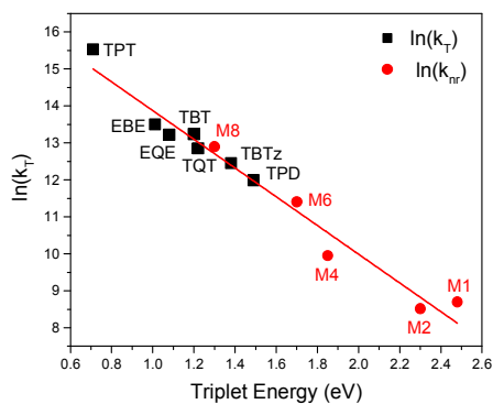
Fig 8 The natural log of the triplet decay rate ( k_T ) of the studied DAD molecules (black squares) and the natural log of the non-radiative decay rate of triplet state from Köhler et al. 19 work (red circles) are plotted against the triplet energy. The straight line corresponds to the linear fitting.
