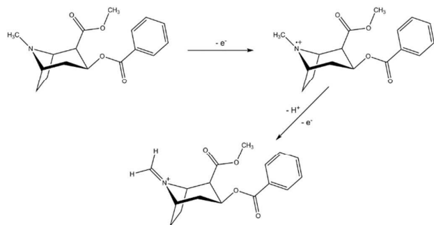
Scheme 1: Oxidation process of cocaine at a carbon screen-printed electrode at potential 1.04 V. The second reaction occurs immediately after the formation of the intermediate radical, causing only one visible peak in a square-wave voltammogram.
