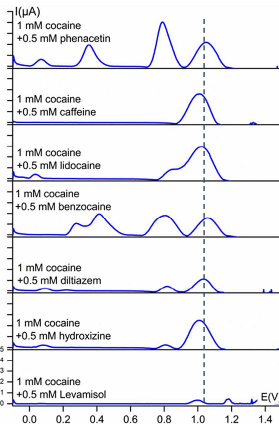
Figure 3: Baseline-corrected square-wave voltammetric responses (vs. Ag/AgCl) of 1 mM solutions of cocaine with 0.5 mM cutting agent at bare carbon screen-printed electrodes in 0.1 M KCl + 0.020 M \text{KH}_2\text{PO}_4 buffer (pH 7). The dotted line represents the characteristic oxidation potential of cocaine at 1.04 V. The y-axis has the same scale in every voltammogram.
