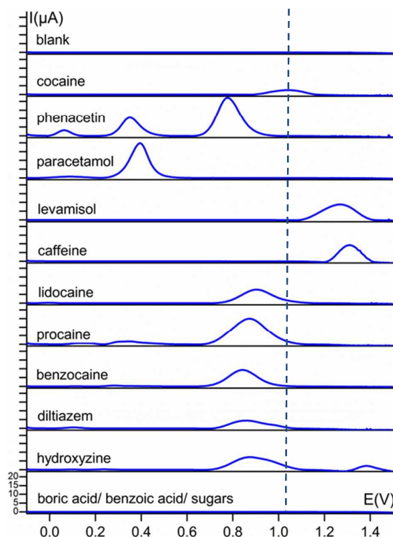
Figure 2: Baseline-corrected square-wave voltammetric responses (vs. Ag/AgCl) of 1 mM solutions of cocaine and cutting agents at bare carbon screen-printed electrodes in 0.1 M KCl + 0.020 M \text{KH}_2\text{PO}_4 buffer (pH 7). The dotted line represents the characteristic oxidation potential of cocaine at 1.04 V. The y-axis has the same scale in every voltammogram.
