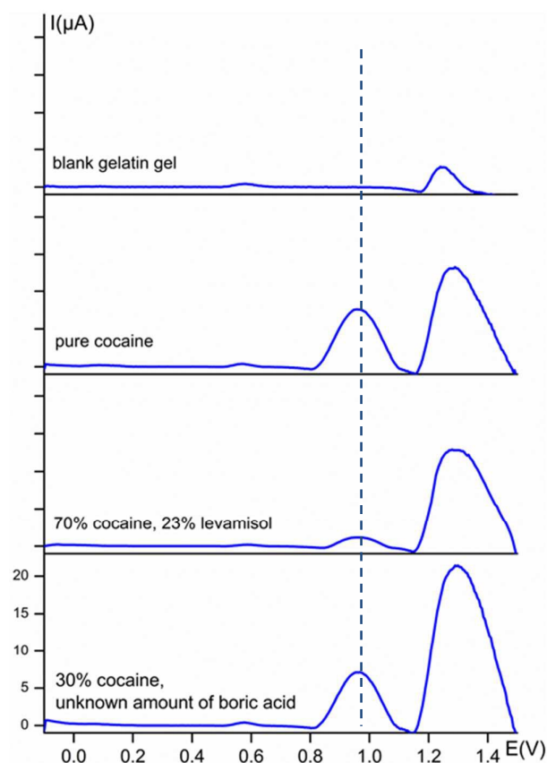
Figure 5: Baseline-corrected square-wave voltammetric responses (vs. Ag/AgCl) of powder street samples at bare carbon screen-printed electrodes using a gelatin gel B hydrogel containing 0.1 M KCl + 0.020 M \text{KH}_2\text{PO}_4 buffer solution (pH 7) as electrolyte. The dotted line represents the oxidation potential of cocaine at 0.97 V. The y-axis has the same scale in every voltammogram.
