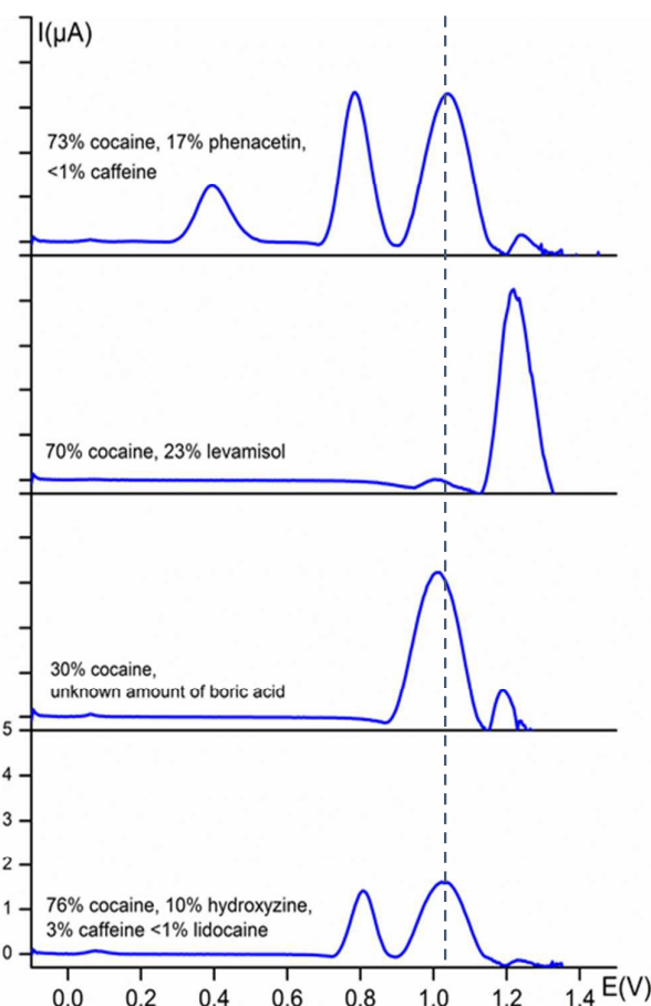
Figure 4: Baseline-corrected square-wave voltammetric responses (vs. Ag/AgCl) of street samples at bare carbon screen-printed electrodes in 0.1 M KCl + 0.020 M \text{KH}_2\text{PO}_4 buffer solution (pH 7). The dotted line represents the characteristic oxidation potential of cocaine at 1.04 V. The y-axis has the same scale in every voltammogram. Each solution was prepared in such way that it contains 1 mM of cocaine.
