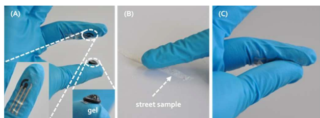
Figure 1: Schematic of the measuring procedure for suspicious powder samples at a wearable fingertip device. (A) The fingertip exhibiting the surface of screen-printed electrode onto a flexible nitrile finger cot (bottom left inset), as well as a conductive gel immobilized upon the thumb (bottom right inset); (B) swiping method of sampling to collect the target powder directly onto the electrode; (C) completion of the electrochemical cell by joining the index finger with electrodes to the thumb coated with the conductive gel electrolyte.
