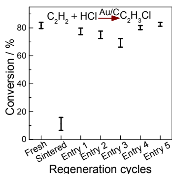
Fig. 7 Relative catalytic activity of acetylene hydrochlorination over the Au/C catalyst before and after regeneration cycles with \text{CHI}_3 treatment for five times. Entries 4 and 5: sintered Au/C catalyst regenerated with \text{CHI}_3 containing \text{HAuCl}_4 (0.002 M) at 40 °C.
