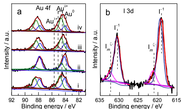
Fig. 3 (a) Au 4f XPS spectra of Au/C catalysts after treatment under different conditions: i) as-prepared; ii) sintered; iii) sintered Au/C treated with \text{CH}_3\text{I} at 40 °C for 30 min; and iv) redispersed Au/C (sample iii) activated by HCl gas at 150 °C for 30 min. (b) I 3d XPS spectra of the redispersed Au/C catalyst (sample iii).
