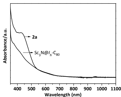
Figure 2. UV-Vis-NIR spectra of \text{Sc}_3\text{N}@I_h\text{-C}_{80} and 2a .
