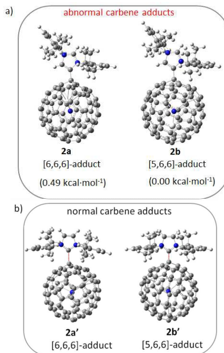
Figure 4. Possible structures of NHC- \text{Sc}_3\text{N}@I_h\text{-C}_{80} complexes and their relative energies calculated at the B3LYP/6-31G*/LANL2DZ (Sc) level.
