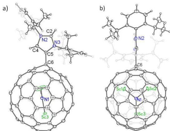
Figure 3. Single-crystal X-ray structure of 2a : (a) side view, (b) front view. Thermal ellipsoids are shown at the 50% probability level. Solvent molecules are omitted for clarity.
