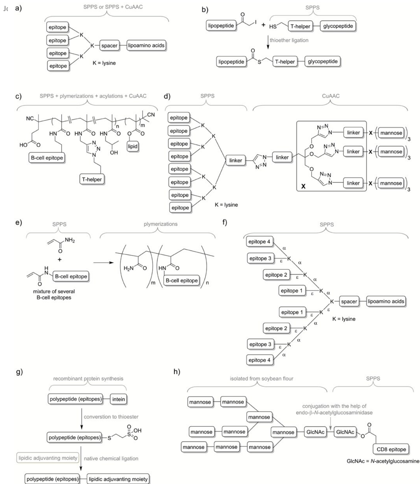
Fig. 4 Examples of peptide-based vaccines and synthetic techniques used for their production: a) lipid core peptide vaccine delivery system (produced by SPPS, occasionally with help of CuAAC); b) vaccine produced with help of thioether ligation; c) multicomponent vaccine obtained by polymerization/conjugation approach; d) asymmetrical dendrimer produced with the help of copper-catalysed azide-alkyne cycloaddition; e) multi-epitope construct produced by random polymerisation of several acrylate modified B-cell epitopes; f) multiple different B-cell epitopes incorporated into one entity via stepwise SPPS using lysine-based branching; g) recombinant polyepitope conjugated to adjuvanting moiety with the help of intein and native chemical ligation; h) glycopeptide-based antigen synthesised in a mixed chemical/enzymatic approach.
