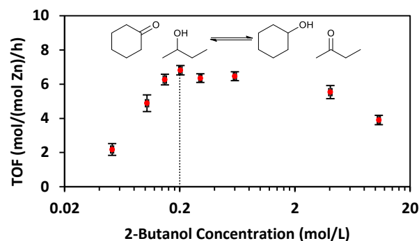
Fig. 4: Initial TOF of MPVO reactions of cyclohexanone and 2-butanol catalyzed by CIT-6 as a function of 2-butanol concentration. Reaction conditions: 100 °C, 0.2 M cyclohexanone, indicated concentration of 2-Butanol in cyclohexane, and 1:100 Zn:cyclohexanone initial molar ratio.
