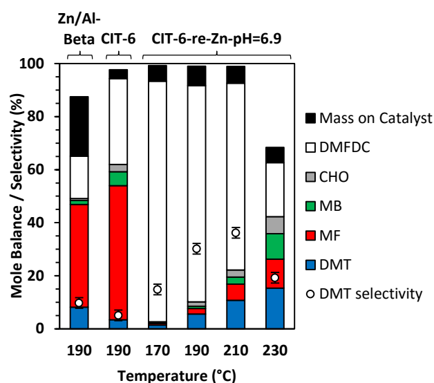
Fig. 6: Diels-Alder cycloaddition-dehydration reactions of DMFDC catalyzed by CIT-6 and CIT-6-re-Zn-pH=6.9 at various temperatures. Resulting yields (%) of DMT, MF, MB, CHO, and DMFDC are calculated as ratio of moles formed to initial moles of DMFDC. Mass on catalyst (%) is expressed as ratio of combustible mass on catalyst (measured by TGA) to initial mass of DMFDC. Reaction conditions: 12h, effective concentration of 0.033M DMFDC in 10 mL heptane, 100 mg of catalyst, and 35 bar C 2 H 2 at 25 °C.
