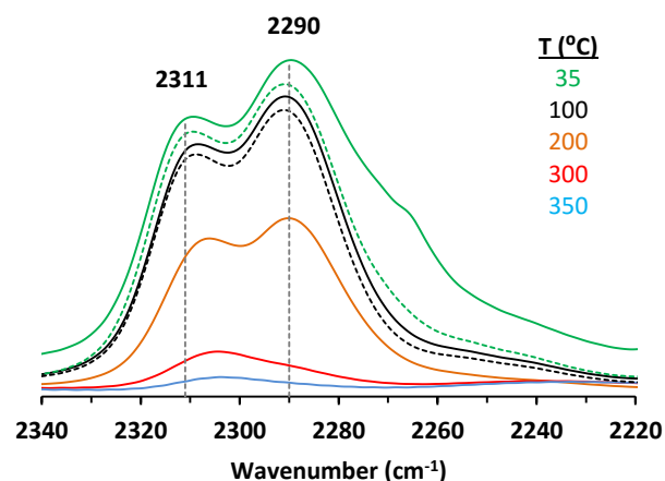
Fig. 2: Baseline corrected IR spectra of CD 3 CN adsorbed on CIT-6 at 35 °C (green solid) and desorbed at different times and temperatures: 24h at 35 °C (green, dashed), 0.5h at 100 °C (black, solid), 1.5h at 100 °C (black, dashed), 0.5h at 200 °C (orange, solid), 0.5h at 300 °C (red, solid), and 0.5h at 350 °C (blue, solid).
