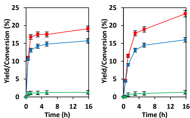
Fig. 3: Glucose isomerization reactions are catalyzed by CIT-6 in water (left) and methanol (right) solvents. Glucose conversion (red squares), fructose yields (blue circles), and mannose yields (green triangles) are plotted as a function of reaction time. Reaction conditions: 100 °C, 1% (wt/wt) glucose, 1:50 Zn:glucose initial molar ratio.
