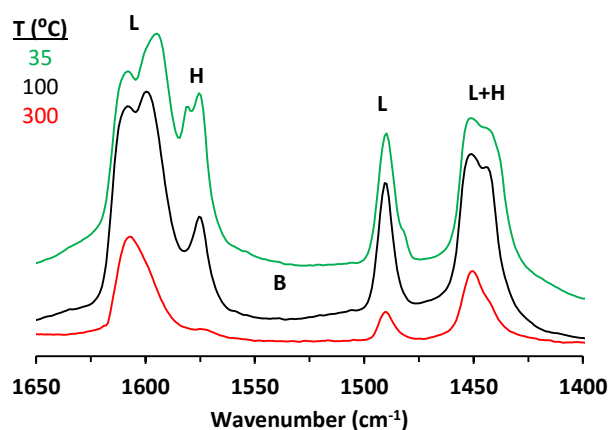
Fig. 1: Baseline corrected IR spectra of pyridine adsorbed on CIT-6 at 35 °C. Different colors (indicated in legend) correspond to different subsequent desorption temperatures carried out for 1h. Peaks corresponding to pyridine coordinated to Lewis acid (L), Brønsted acid (B), and hydrogen-bonding (H) sites are marked.
