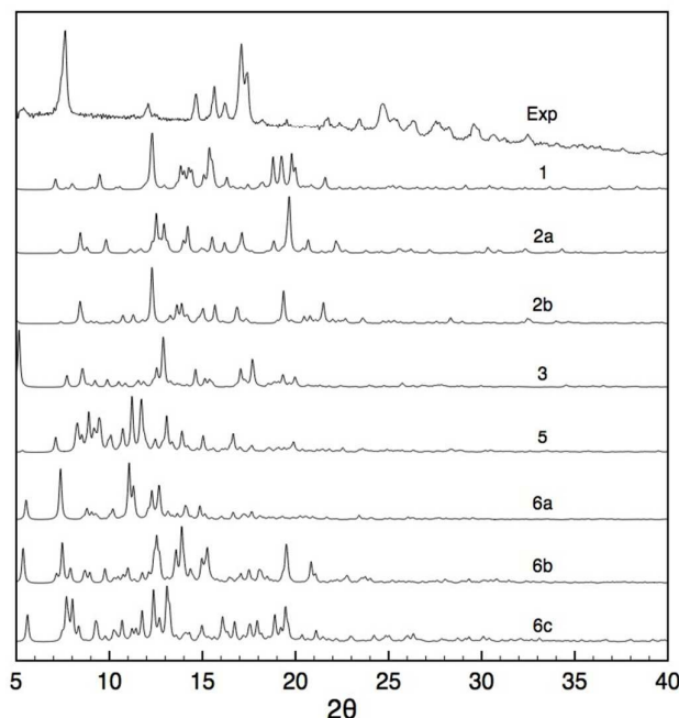
Figure 6. Comparison between the experimental PXRD pattern and the simulated spectra for structures 1-6 after all-atom DFT optimization
