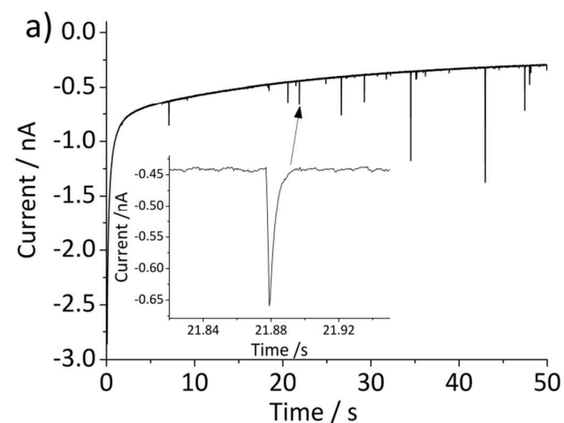
Figure 3. Characteristic chronoamperogram recorded at a gold microelectrode in deoxygenated 20 mM KCl with pre-dispersed hematite nanoparticles at pH 2.1 and at an applied potential of -0.4 V vs. Ag/AgCl. The inset provides an enlarged view of the current-time profiles illustrating the faradaic reduction of nanoparticles upon collision with the working electrode as spikes.
