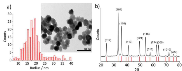
Figure 1. (a) A TEM image of hematite nanoparticles prepared by forced hydrolysis and a histogram illustrating a distribution of particle radius based on 215 individuals with the mean radius of 18.0 \pm 2.5 nm. (b) The powder XRD spectrum of hematite nanoparticles. Peak positions are in good agreement with the reference patterns, PDF#072-0469 25 , which is shown at the bottom of the figure. Miller indexes are assigned to each peak in accordance to Wang et al. 24 for \alpha -Fe 2 O 3 prepared under a similar condition to this study.
