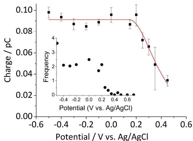
Figure 5. Log normal average reductive charges for individual hematite nanoparticles in deoxygenated 20 mM KCl at pH 2.1 as a function of the applied potential (black square). Error bars indicate the standard error of the mean. The result of nonlinear curve fitting given by Eqn. 10 is shown as red line. Parameters extracted from the fit are r_i = 15.0 \pm 0.1 nm, E_{1/2} = 0.377 \pm 0.17 V vs. Ag/AgCl, (n'+\alpha) = 0.17 \pm 0.03 , and k^0 \exp\left[\frac{(n'+\alpha)E_f}{RT}\right] = 1.17 (\pm 0.42) \times 10^5 mol \text{cm}^{-2} \text{s}^{-1} . The inset shows the impact frequency, i.e. the number of spikes observed per chronoamperogram, as a function of the electrode potential.
