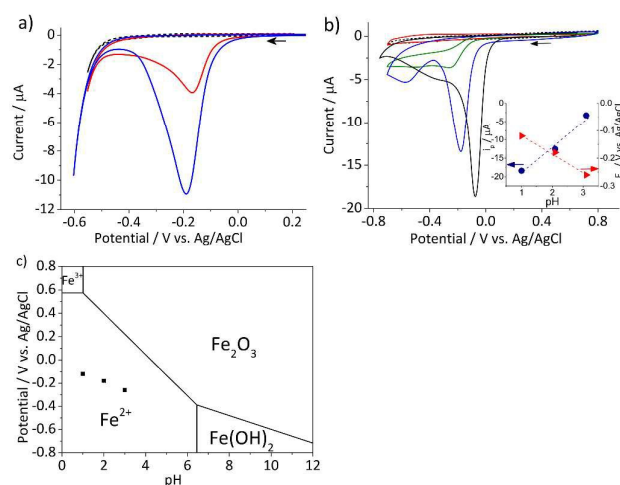
Figure 2. (a) Characteristic cyclic voltammograms of gold electrodes modified with 2.8 \times 10^{-5} \text{ g cm}^{-2} (red) and 5.5 \times 10^{-5} \text{ g cm}^{-2} hematite nanoparticles (blue) and an unmodified gold electrode (black dash) recorded at a scan rate of 0.01 \text{ V s}^{-1} in deoxygenated 20 mM KCl at pH 2.1 adjusted by addition of appropriate amounts of 20 mM HCl. (b) Cyclic voltammograms of glassy carbon electrodes modified with 2.4 \times 10^{-5} \text{ g cm}^{-2} hematite recorded at a scan rate of 0.01 \text{ V s}^{-1} in deoxygenated 20 mM KCl solutions at pH 4.4 (red), 3.1, (green), and 2.1 (blue). A cyclic voltammogram at pH 1 (black solid line) was collected in 0.1 M HCl and that of a bare glassy carbon electrode (black dash) was collected at pH 2.1. The inset shows the plots of the peak current, i_p , (blue circle) and the peak potential, E_p , (red triangle) as a function of pH. (c) The Pourbaix diagram of iron 27 at the ambient conditions, while black squares indicate the peak potentials observed in (b).
