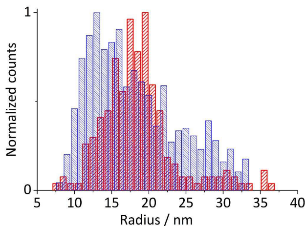
Figure 4. Histogram of particle radius determined from spikes obtained during chronoamperometry at -0.4 V vs. Ag/AgCl and corrected for the diffusion coefficient (blue, dense mesh) and from TEM (red, medium mesh). The mean value of 15.2 \pm 1.8 nm is determined from a log-normal distribution curve of radius resulting from the particle impact.
