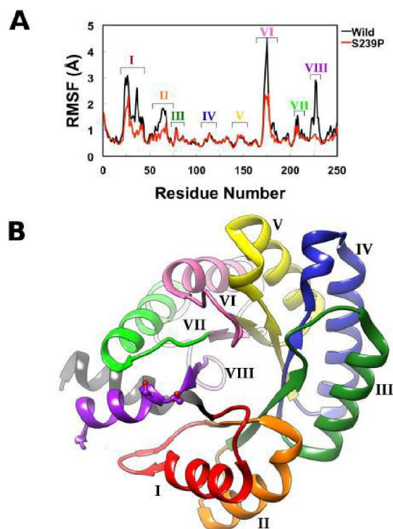
Fig. 5 (A) Average root mean square fluctuations, averaged over all three MD trajectories for wild-type DERA and the S239P mutants. The key peaks on the RMSF plot are colour coded on the protein in panel (B).
