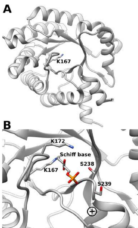
Fig. 2 (A) (\alpha/\beta)_8 TIM barrel structure of DERA, highlighting the active-site Lys 167 that forms the Schiff base with the incoming aldehyde (dR5P or acetaldehyde). (B) Close-up of the DERA active site, with the Lys 167 -dR5P complex shown in a stick representation. The side-chains of Ser 238 (two conformers in the crystal structure) and Ser 239 and Lys 172 are shown in sticks. The "plus" indicates the location of the N-terminus of \alpha -helix 8. Image created with Chimera 6 using the atomic coordinates in PDB ID 1JCJ 7,8 .
