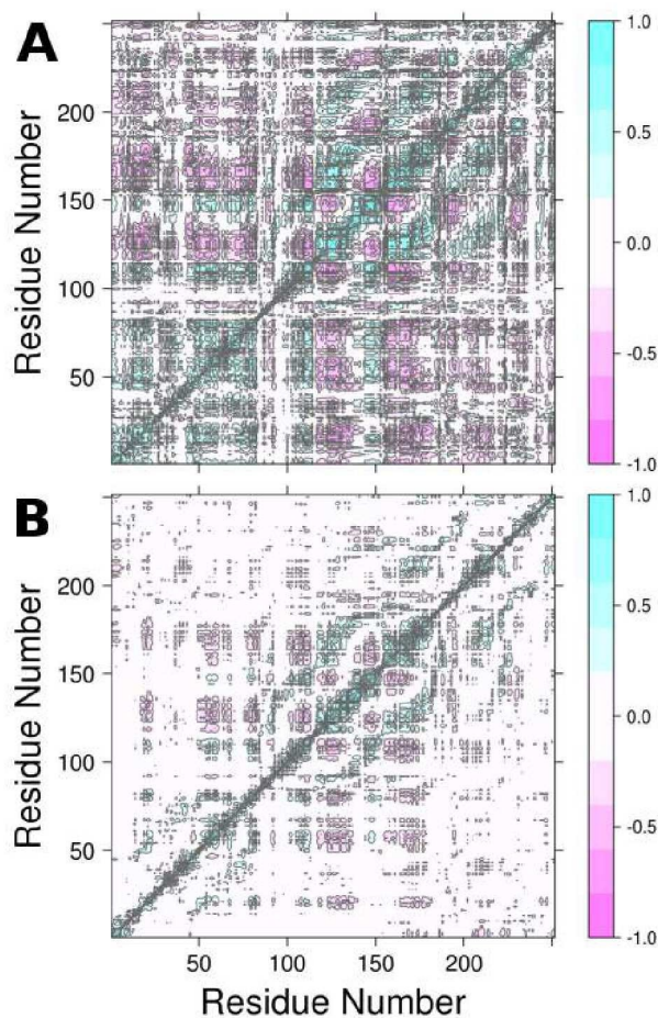
Fig. 6 Dynamic cross correlation maps (DCCM) of (A) wild-type DERA and (B) the S239P mutant. Corresponding DCCM plots for all mutants can be found in Fig. S5. This Fig. was generated using Bio3D 29,30 .
