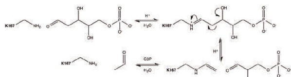
Fig. 1 Mechanism of the DERA catalysed aldol cleavage of dR5P. The side-chain amine of Lys 167 condenses with the incoming aldose to form the imine equivalent. The imine facilitates C-C bond cleavage between carbons 2 and 3 by resonance stabilization of the resulting carbanion. The Schiff base stabilizes the enamine formed by either the catalysed cleavage of an aldol to the respective components, or by the deprotonation of the \alpha -proton of a donor aldimine (or ketimine) during the aldol addition reaction. The catalytic cycle is completed by hydrolysis of the enamine. Auxiliary catalytic residues have been omitted for clarity.
