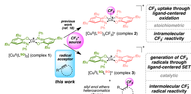
Figure 1. Ligand-based redox reactivity of complex 1 with an electrophilic \text{CF}_3^+ source.
