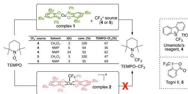
Scheme 1. TEMPO trapping experiments for the generation of \text{CF}_3^\bullet radicals with complexes 1 and 2. NMP: N-methylpyrrolidinone.
