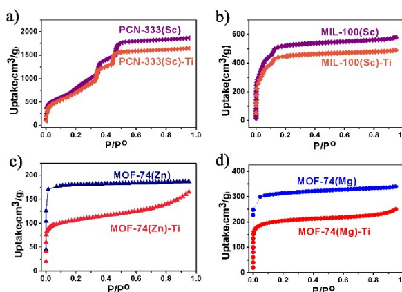
Fig. 3 \text{N}_2 uptakes for template MOFs and the corresponding titanium MOFs at 77K, 1 atm.
