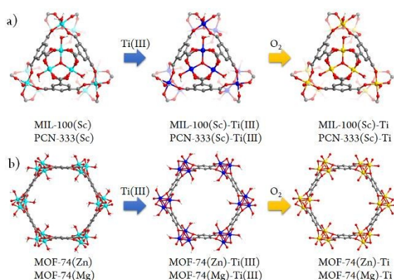
Fig. 1 Schematic illustration of the stepwise HVMO procedure for the design of Ti-MOFs from the template MOFs: a) MIL-100(Sc) and PCN-333(Sc) metal metathesis with Ti(III), followed by metal node oxidation in the air (PCN-333(Sc) and MIL-100(Sc) have same topology but different structures); b) similar process for MOF-74(Zn) and MOF-74(Mg).
