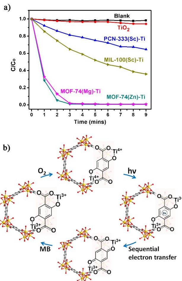
Fig. 5 a) Photodegradation of MB using no catalyst (blank), TiO_2 , PCN-333(Sc)-Ti, MIL-100(Sc)-Ti, MOF-74(Zn)-Ti and MOF-74(Mg)-Ti with 300 W Xenon light irradiation; b) Proposed mechanism of MB degradation of Ti-MOF-74 in the presence of air.
