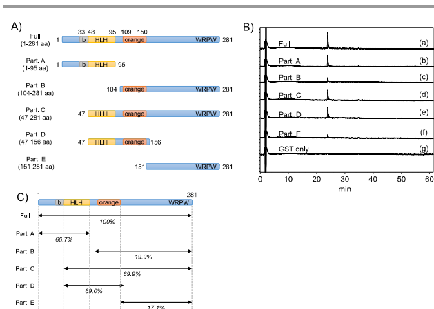
Figure 8. The binding ability of compound 2 to Hes1 partial proteins. All GST-Hes1 proteins were used ca. 3.6 nmol and GST protein was used ca. 3.8 nmol. A) Schematic showing of synthesized Hes1 full and partial proteins. B) The results of binding amount of compound 2 to each protein beads. (a) GST-Hes1 (1-281 aa) beads, (b) GST-Hes1 (1-95 aa) beads, (c) GST-Hes1 (104-281 aa) beads, (d) GST-Hes1 (47-281 aa) beads, (e) GST-Hes1 (47-156 aa) beads, (f) GST-Hes1 (151-281 aa) beads, (g) GST beads. The mass of binding compound were calculated from the area of the peaks. C) The predicted binding ability from the results of beads assay.
