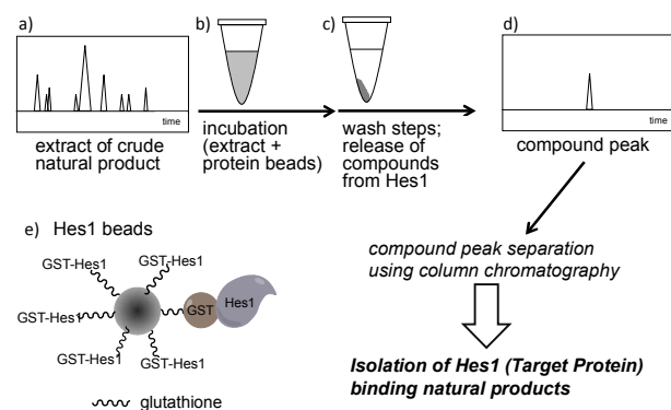
Fig. 1 Schematic showing target protein-oriented natural product isolation by the Hes1 beads-HPLC method. a) HPLC profile of a natural product extract; b) incubation of the extract with Hes1 beads; c) washing the beads and release of compounds from Hes1; d) detection of the Hes1 binding natural product; e) representation of the Hes1 glutathione Sepharose beads.
