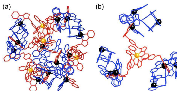
Figure 6. Left: View of the complete complex cation of [Ru 4 Cd 12 (L ph ) 12 (L naph ) 12 ](PF 6 ) 7 (BF 4 ) 25 , (same colouring scheme as Fig. 4). Right: Partial view of the complex, emphasising how each fac -[Ru(L ph ) 3 ] 2+ vertex is connected to three [Cd 3 (L naph ) 3 ] 6+ units.
