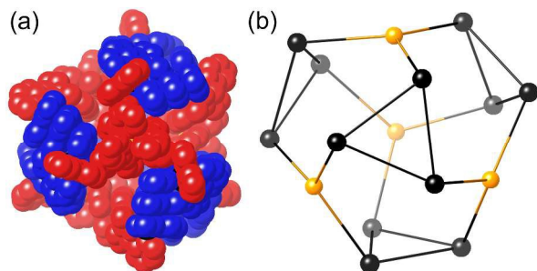
Figure 4. Two views of the crystal structure of [Ru 4 Cd 12 (L ph ) 12 (L naph ) 12 ](PF 6 ) 7 (BF 4 ) 25 . (a) The entire complex cation in spacefilling view (L naph shown in blue, L ph shown in red); (b) arrangement of metal ions in the Ru 4 Cd 12 core (Ru – yellow, Cd – black).
