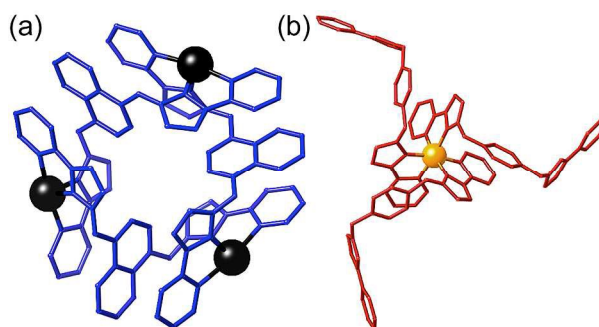
Figure 5. Fragments from the crystal structure of [Ru 4 Cd 12 (L ph ) 12 (L naph ) 12 ](PF 6 ) 7 (BF 4 ) 25 (same colouring scheme as Fig. 4). (a) A [Cd 3 (L naph ) 3 ] 6+ triangular cyclic helicate unit; (b) a fac -[Ru(L ph ) 3 ] 2+ unit.
