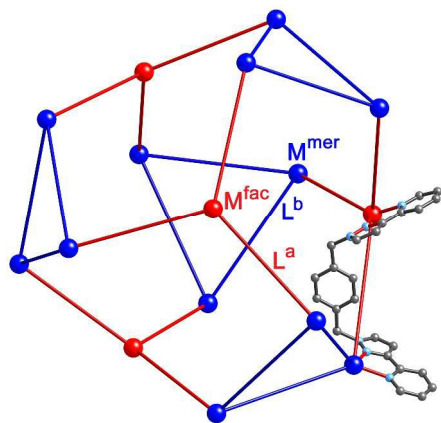
Figure 2 Representation of the core structure of [Cd_{16}(L^{ph})_{24}](ClO_4)_{32} (ref. 5) with one bridging ligand included. All metal sites are Cd(II) but the two different types of geometric isomer are colour-coded: fac tris-chelate metals are in red ( M^{fac} , see main text) and mer tris-chelate metals are in blue ( M^{mer} ). Likewise the two ligand environments are L^a in red, and L^b in blue (see main text).
