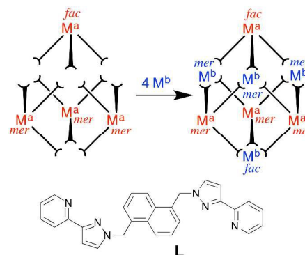
60 Figure 1. Example of stepwise preparation of heterometallic cages from a mixture of kinetically inert units [(M^a)L_3]^{2+} and additional labile ions (M^b)^{2+} in a 4:4 stoichiometry (from ref. 4).
