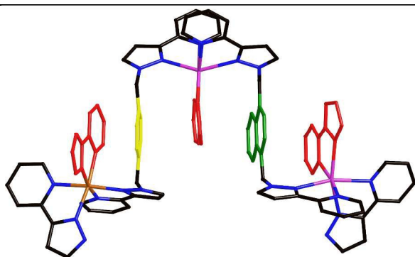
Figure 7. Five-layer aromatic stack in the structure of [\text{Ru}_4\text{Cd}_{12}(\text{L}^{\text{ph}})_{12}(\text{L}^{\text{naph}})_{12}](\text{PF}_6)_7(\text{BF}_4)_{25} with electron-rich phenyl and naphthyl rings in yellow and green, respectively, and electron deficient pyrazolyl-pyridine units in red. Cd – purple; Ru – orange.
