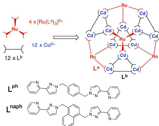
Figure 3. Sketch of the stepwise synthetic strategy used in this work to prepare the heterometallic, mixed-ligand cage: viz combination of pre-formed fac -[Ru(L a ) 3 ] 2+ (red), additional labile Cd 2+ ions (blue), and free ligand (L b , black) in a 4:12:12 ratio to give hexadecanuclear [Ru 4 Cd 12 (L a ) 12 (L b ) 12 ] 32+ with L a = L ph and L b = L naph .
