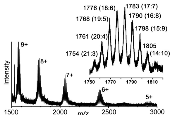
Figure 9 Partial electrospray mass spectrum of redissolved crystals of [\text{Ru}_4\text{Cd}_{12}(\text{L}^{\text{ph}})_{12}(\text{L}^{\text{naph}})_{12}](\text{PF}_6)_7(\text{BF}_4)_{25} showing the sequence of signals associated with progressive loss of anions. For each charge, the presence of multiple closely-spaced signals is associated with different combinations of [\text{BF}_4]^- and [\text{PF}_6]^- anions. The inset shows the expansion of the set of signals around m/z 1780 for the 8+ ions: the number of [\text{BF}_4]^- and [\text{PF}_6]^- anions for each is shown in parentheses. Thus, the signal at m/z 1768 corresponds to \{[\text{Ru}_4\text{Cd}_{12}(\text{L}^{\text{ph}})_{12}(\text{L}^{\text{naph}})_{12}](\text{BF}_4)_{19}(\text{PF}_6)_5\}^{8+} , etc. For high-resolution expansions, see ESI.
