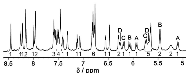
Figure 8. ^1\text{H} NMR spectrum ( \text{CD}_3\text{NO}_2 , 800 MHz) of redissolved crystals of [\text{Ru}_4\text{Cd}_{12}(\text{L}^{\text{ph}})_{12}(\text{L}^{\text{naph}})_{12}](\text{PF}_6)_7(\text{BF}_4)_{25} . Integers under the signals are integral values (total 42). Labels A – D refer to the four pairs of doublets from diastereotopic methylene groups, identified from a COSY spectrum, which confirm the presence of two independent ligand environments with no internal symmetry and equal numbers of each type (see main text).
