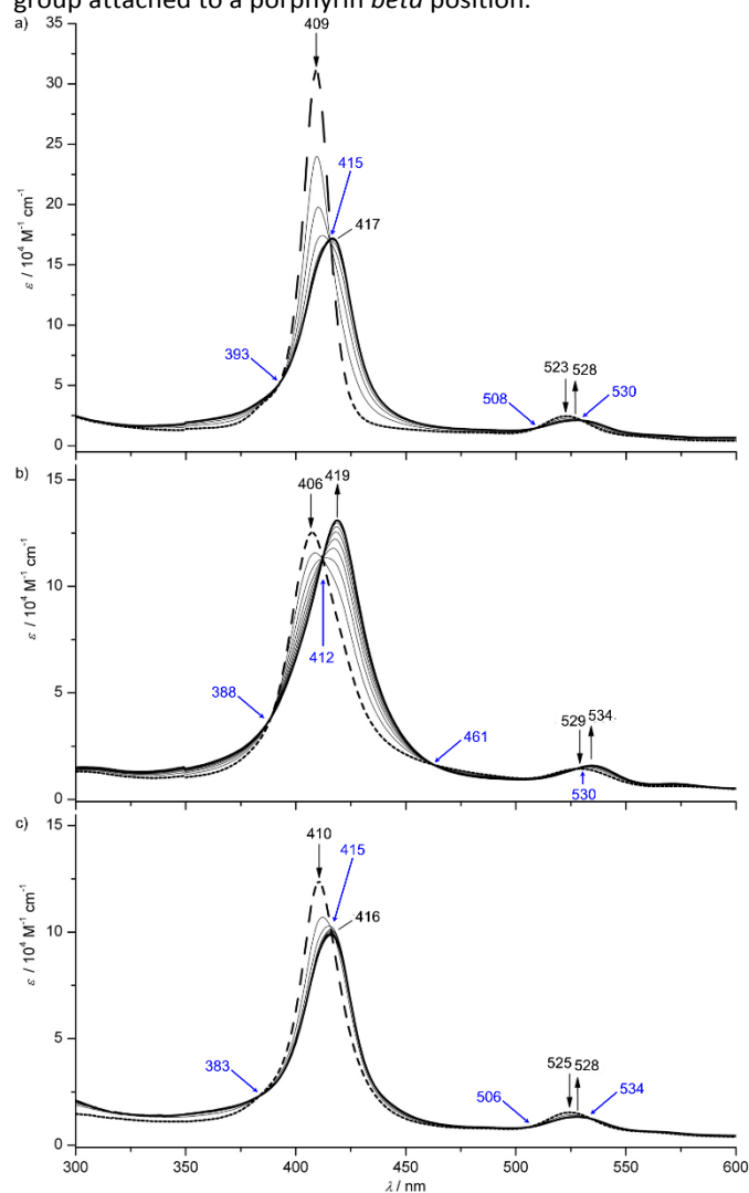
Fig. 3 UV/Vis spectral changes upon the first electroreduction of a) [1a]^+ , b) [2a]^+ and c) [3a]^+ in 0.1 M [tBu_4N][PF_6] /THF solution (isosbestic points indicated in blue).
