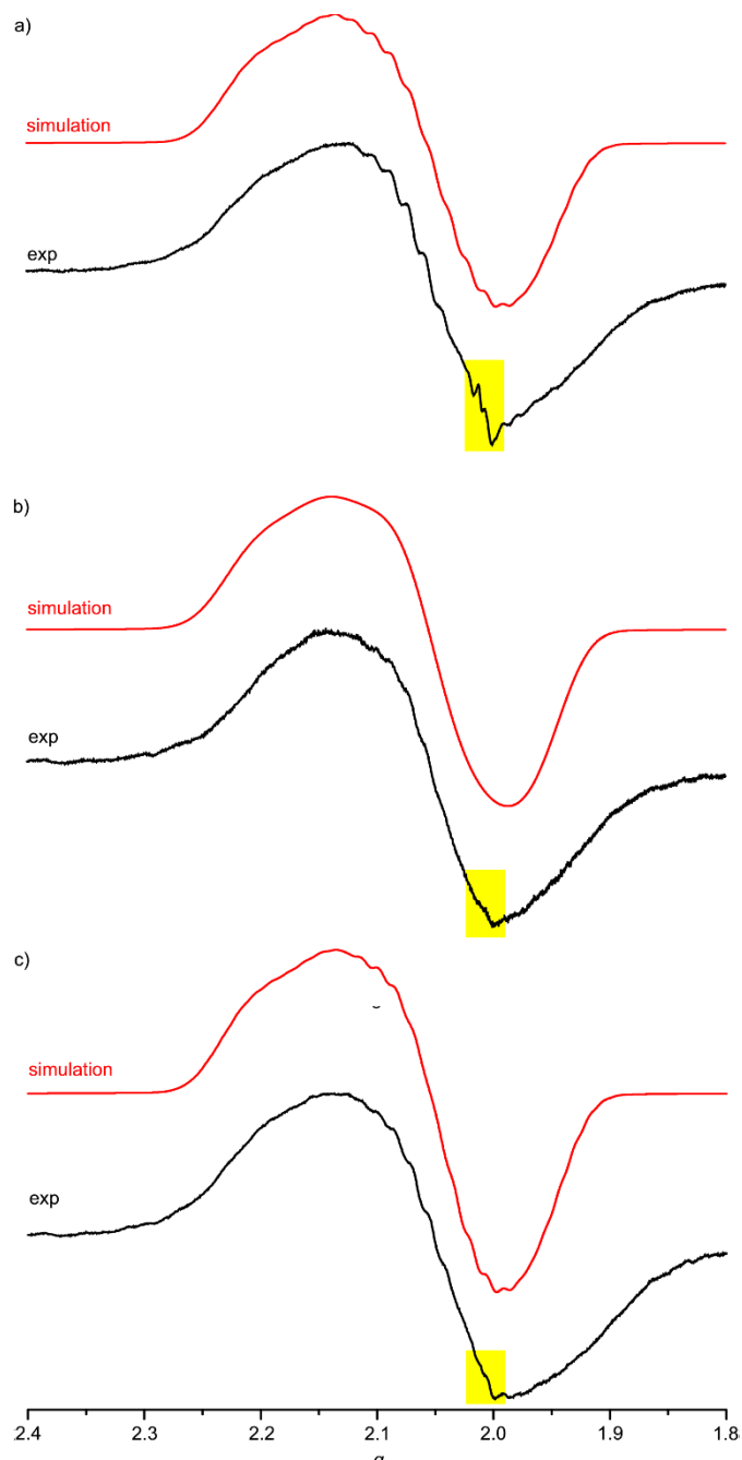
Fig. 6 X-band EPR spectra of a) 4a (MeOH), b) 4b (THF) and c) 4c (THF) in frozen solution (77 K, 9.4 GHz) and corresponding simulations; yellow squares highlight the presence of traces of porphyrin radical anions 4a' , 4b' and 4c' , respectively.
