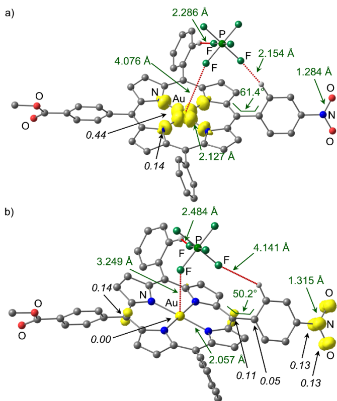
Fig. 8 Spin densities of DFT optimised geometries of a) [1a^-PF_6]^- and b) [1a'^-PF_6]^- (isosurface value at 0.01 a.u. in yellow; UB3LYP, LANL2DZ, IEFPCM CH_2Cl_2 ; hydrogen atoms which are not involved in hydrogen bonds are omitted; Mulliken spin densities in italics).
