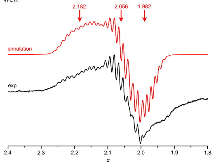
Fig. 4 X-band EPR spectrum of \text{Au}(\text{TPP}) in frozen \text{CH}_2\text{Cl}_2 solution (77 K, 9.4 GHz) and corresponding simulation.
