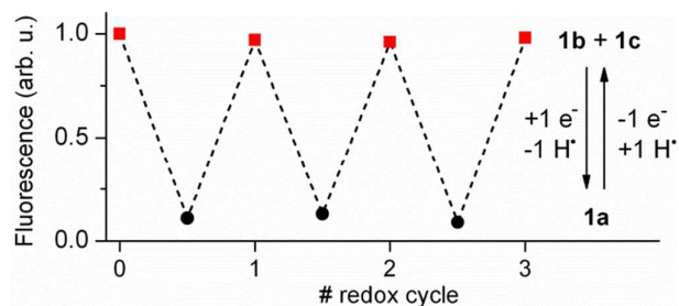
Fig. 4 Fluorescence intensity of 1 in acetonitrile at 298 K ( 5 \times 10^{-3} M + 0.1 M n\text{-Bu}_4\text{NPF}_6 ) upon consecutive exhaustive electrolysis (1 F, 2.41 C) at E_{\text{sp}} = -1.00 V and +1.00 V (vs SCE) to induce reversible interconversion between 1b+1c and 1a via reduction and oxidation processes, respectively. In the redox conversion of 1a into 1b+1c , the solvent (e.g. acetonitrile) is used as the source of hydrogen atoms.
