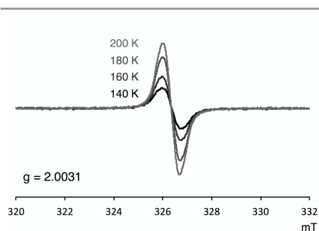
Fig. 5 VT ESR spectra of 1a in solid state.
