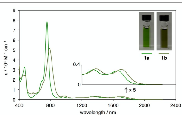
Fig. 6 UV-vis-NIR absorption spectra and photographs of CS 2 solution (ca. 1 \times 10^{-4} M) of 1a and 1b .
