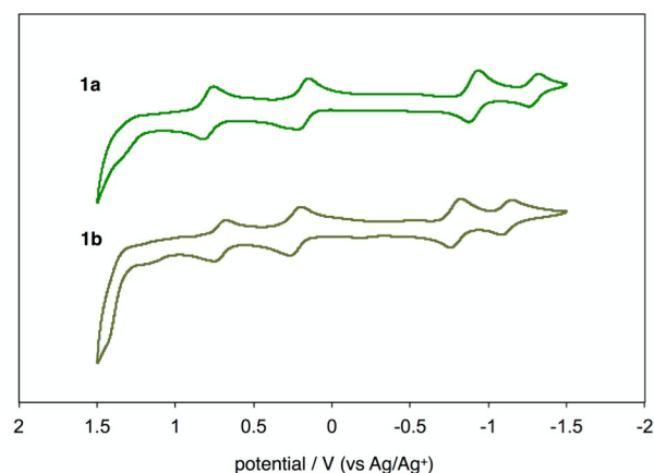
Fig. 7 Cyclic voltammograms of 1a and 1b in CH 2 Cl 2 with n -Bu 4 N + (CF 3 SO 2 ) 2 N - as supporting electrolyte, and scan rate of 0.1 V/s.
