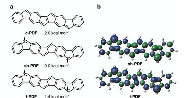
Fig. 2 (a) Electronic states of PDF with energy values relative to the most stable states. (b) Spin density distributions. Blue and green surfaces represent a and b spin densities, respectively. Isovalue is 0.003. Calculated at the (U)B3LYP/6-311+G(d,p) level.
