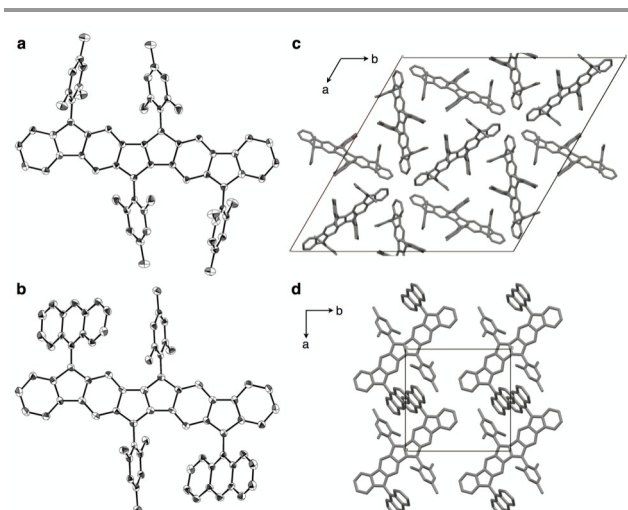
Fig. 4 ORTEP drawings of 1a (a) and 1b (b) with 50% probability (all hydrogen atoms and solvent molecules are omitted for clarity; half of the entire structure constitutes an asymmetric unit), and packing structure of 1a (c) and 1b (d) along c axis.
