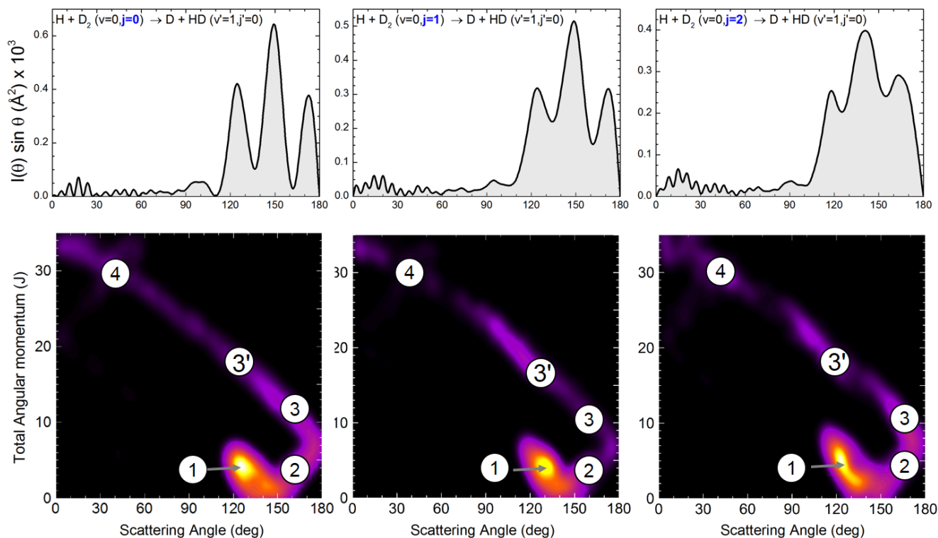
FIG. 2: Angular distributions and deflection functions for the \text{H} + \text{D}_2(v=0, j=0-2) \rightarrow \text{D} + \text{HD}(v'=1, j'=0) reaction at 1.97 eV collision energy. The top panels show the QM angular distributions for the three rotational states populated in the experiment. The bottom panel shows the state-to-state quasiclassical deflection functions, D, (J, \theta) . Although the oscillation pattern is clearly affected by the initial rotational state, the QCT deflection functions are remarkably similar. The quasiclassical mechanisms are labelled in the figure as 1 (ear), 2, 3, 3' and 4 (the last three form the spiral). 25, 26 The spiral mechanism displays a clear correlation between J and \theta that extends over the whole range of scattering angles. The sketches of the mechanisms that correspond to the labelled regions of D, (J, \theta) are displayed in the Fig. S1.
