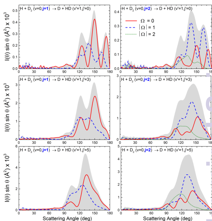
FIG. 3: QM DCS( |\Omega| ) for the \text{H} + \text{D}_2(v=0, j=1-2) \rightarrow \text{D} + \text{HD}(v'=1, j') reactions. The interference pattern, partially blurred as j increases, clearly reappears when the contributions due to the different |v, j, \Omega\rangle states are separated.
