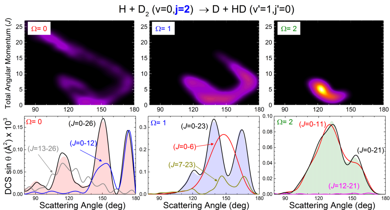
Fig. 4: Origin of multiple peaks in backward scattering of \text{HD}(v'=1, j'=0, \Omega) products for initial j=2 . The top panels show the joint QCT J - \theta deflection function resolved in \Omega , (2J + 1) P_r(J, \theta; \Omega) \sin \theta , analogous to that displayed in the panel (b) of Fig. 1. The bottom panels show the decomposition of the QM angular distributions from the contributions of various sets of J . The notation \text{DCS}(J_1 - J_2) means that the DCS is constructed by including partial waves in the range [J_1, J_2] including the respective cross terms. The global \text{DCS}(|\Omega|) is depicted as a shaded background.
