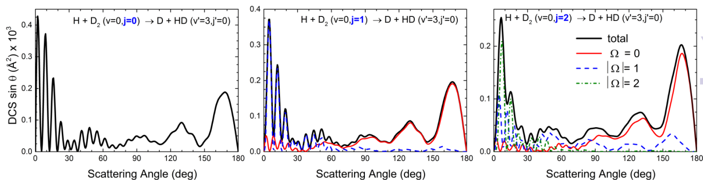
FIG. 5: QM DCS( |\Omega| ) and angular distributions and deflection functions for the \text{H} + \text{D}_2(v=0, j=0-2) \rightarrow \text{D} + \text{HD}(v'=3, j'=0) reaction.
