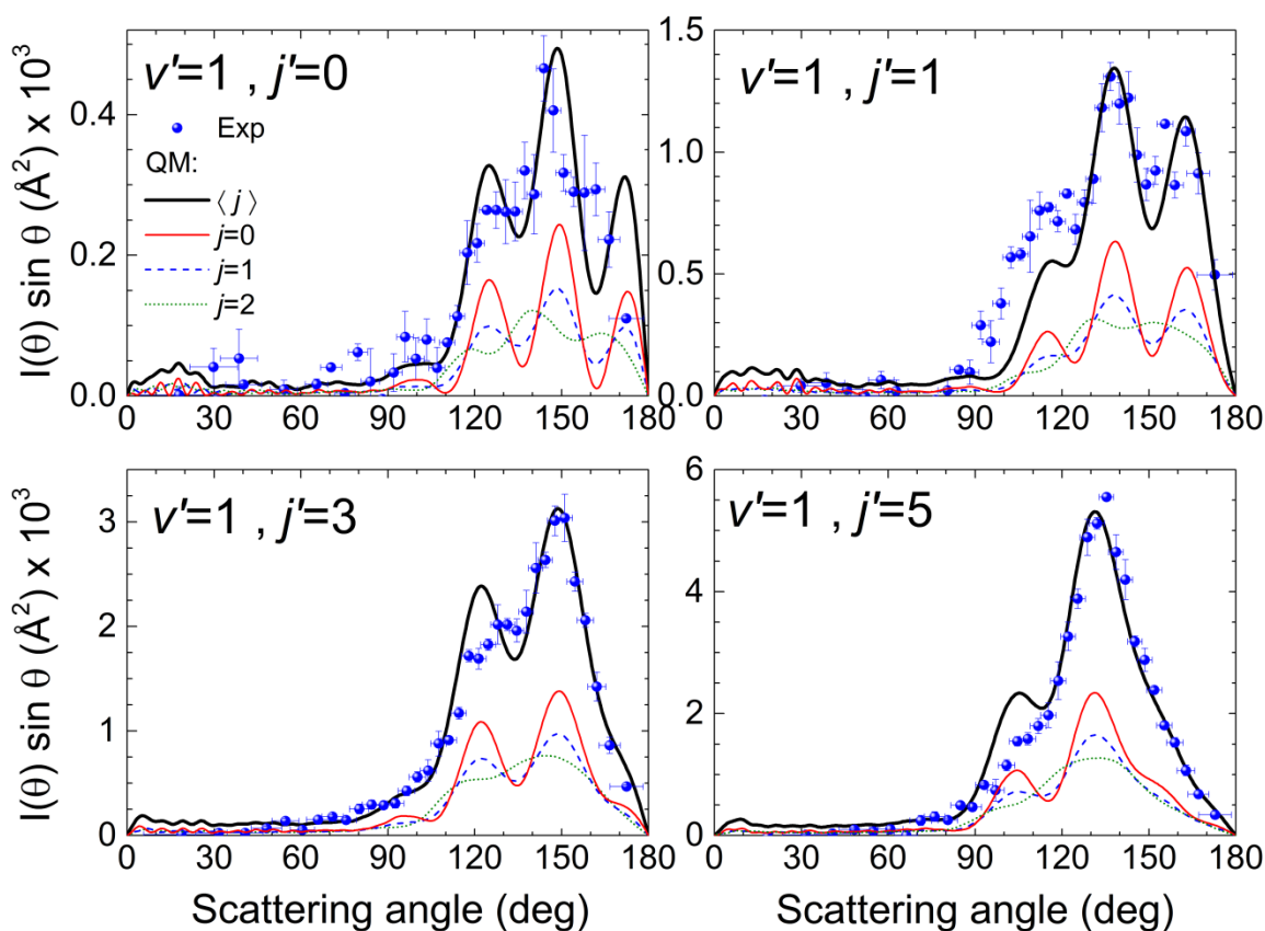
FIG. 1: Comparison between the experimental angular distributions (blue solid circles) and their theoretically simulated counterparts (continuous black line) for four HD( v' , j' ) rovibrational states at 1.97 eV mean collision energy. The simulation implies the averaging of the differential cross sections (multiplied by \sin \theta ) over the experimental collision energy distribution and angular resolution. The simulation also implies to take into account the weighted contributions from the reaction with D_2 in the rotational states populated under the experimental conditions. The corresponding contributions are indicated in each panel by red line ( j=0 ), blue line ( j=1 ) and green line ( j=2 ) such that their sum yields the black line.
