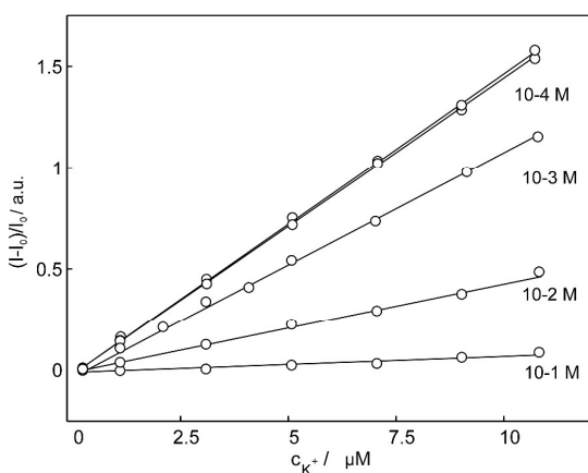
Figure 8. Observed linear calibration curves of normalized fluorescence response of nanospheres based on 18C6 to the potassium cation at different sodium background levels.
