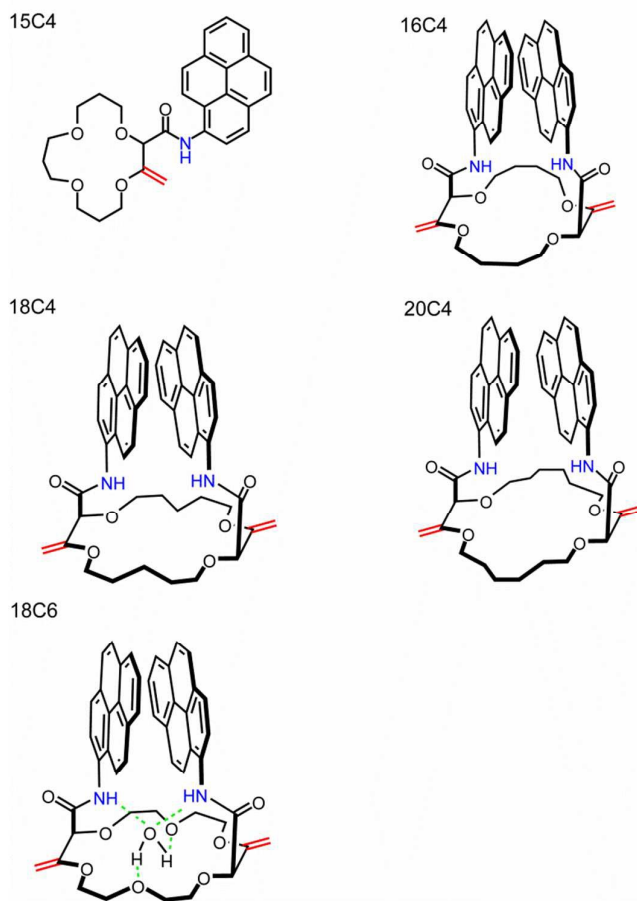
Figure 2. Structures of the studied polyether macrocycles.
