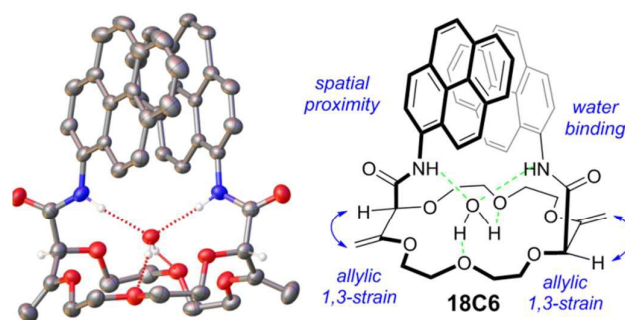
Figure 1. "Dixial"-like conformation of 18C6. Displacement ellipsoid plot of the crystal structure drawn at 50% probability. Only one of the four superimposable macrocycles present in the asymmetric unit is depicted. A solvent molecule is also omitted for clarity.
