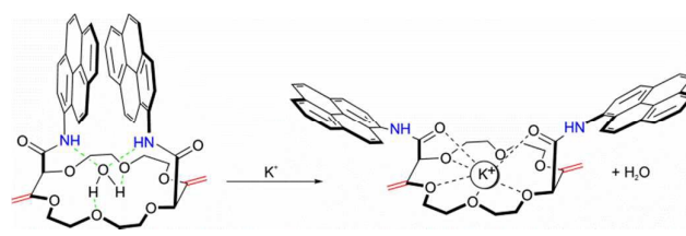
Figure 7. Proposed sensing mechanism of binding of potassium to 18C6, resulting in a conformational change.
