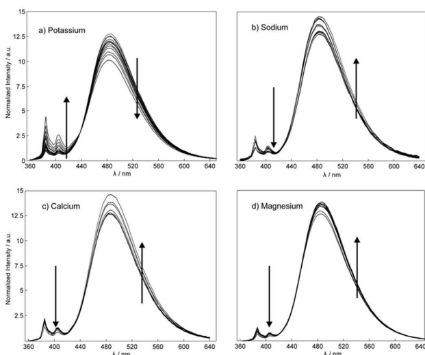
Figure 6. Effect of the addition of different cations on the fluorescence emission behavior of \text{K}^+ selective nanospheres ( \lambda_{\text{excitation}} = 346 nm) in the concentration range 10^{-6} to 10^{-1} M.
