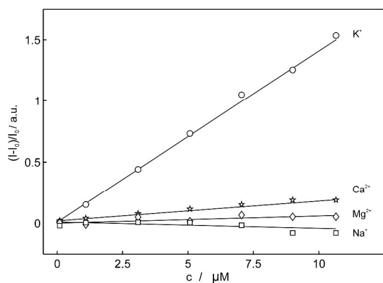
Figure 5. Observed linear calibration curves of normalized fluorescence at 406 nm as a function of concentration of different cations for 18C6 ( \lambda_{\text{excitation}} = 346 nm).
