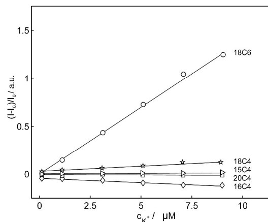
Figure 4. Observed linear calibration curves of normalized fluorescence at 406 nm as a function of potassium concentration for different macrocyclic compounds (15C4, 16C4, 18C4, 18C6, 20C4) in exhaustive fluorescence mode ( \lambda_{\text{excitation}} = 346 nm).
