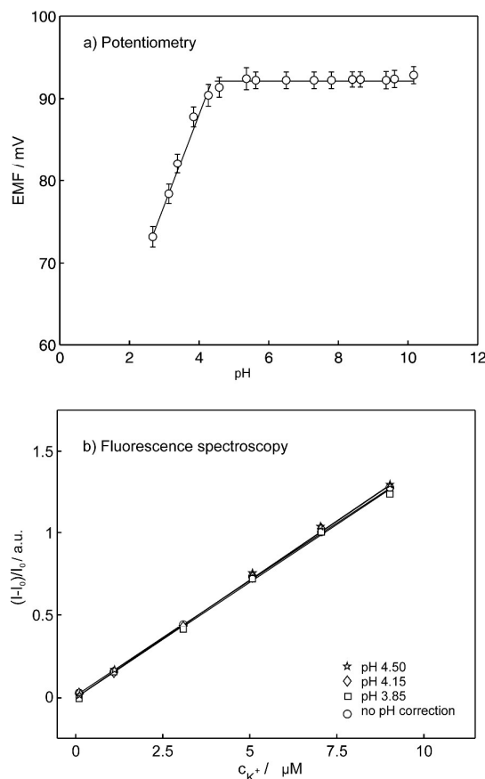
Figure 9. (a) Potentiometric response of the potassium selective sensor to the changes in concentration of H^+ at fixed concentration of potassium 1 mM and (b) observed linear calibration curves from the normalized fluorescence spectra as a function of potassium concentration at different pH.
