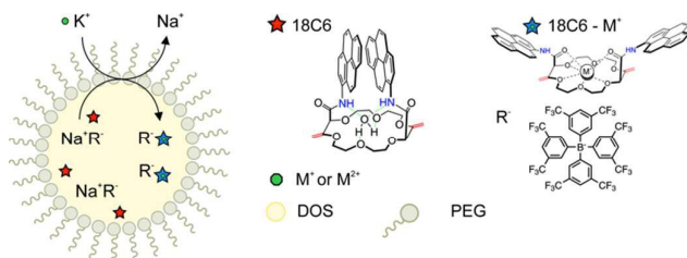
Figure 3. Ion-selective emulsions doped with macrocyclic compound as an ionophore, a plasticizer DOS and the hydrophobic structure of PEG. The sensing mechanism is based on ion-exchange between the target ion \text{K}^+ in aqueous phase and the counter ion \text{R}^- in the organic phase (1) and the specific reaction between 18-crown-6 compound (18C6) and the ion of interest (2).
