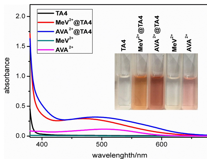
Fig. 6 UV-vis absorption spectra (1.0 mM, 25 °C) of \text{TA}4 , \text{MeV}^{2+}\text{-}2\text{PF}_6 , \text{AVA}^{2+}\text{-}2\text{PF}_6 , \text{MeV}^{2+}\text{-}2\text{PF}_6@\text{TA}4 , and \text{AVA}^{2+}\text{-}2\text{PF}_6@\text{TA}4 . Inset: the photo of the above solutions.
