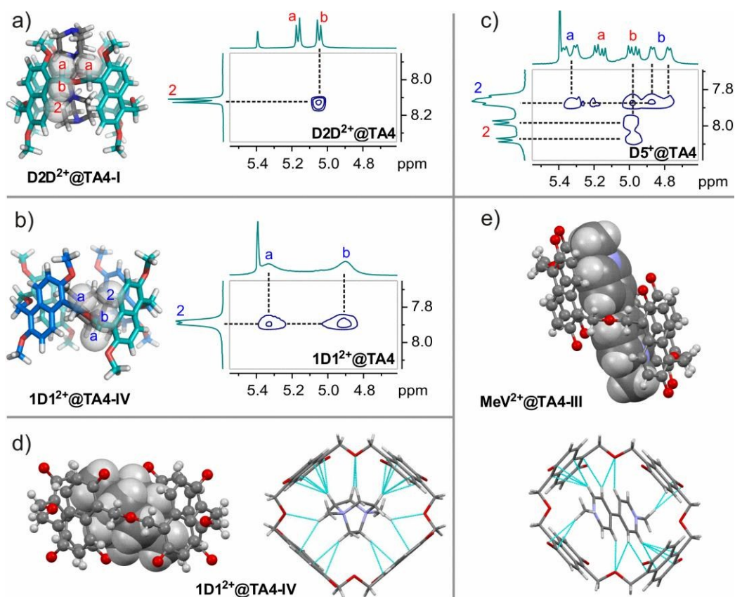
Fig. 4 Energy-minimized structures and partial ^1\text{H} , ^1\text{H} -ROESY NMR spectra (500 MHz, \text{CD}_2\text{Cl}_2:\text{CD}_3\text{CN} = 1:1 , 6.0 mM, 25 °C) of (a) \text{D}2\text{D}^{2+}@\text{TA}4\text{-I} , (b) 1\text{D}1^{2+}@\text{TA}4\text{-IV} , and (c) \text{D}5^{+}@\text{TA}4 . The protons a , b , a' , b' , 2' , and 2 in the models are rendered to show possible NOE contacts; Single crystal structures of (d) \text{MeV}^{2+}@\text{TA}4\text{-III} and (e) 1\text{D}1^{2+}@\text{TA}4\text{-IV} . Butyl groups are removed for viewing clarity.
