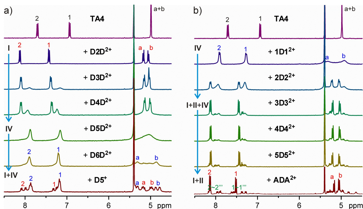
Fig. 3 Partial ^1\text{H} NMR spectra (400 MHz, \text{CD}_2\text{Cl}_2:\text{CD}_3\text{CN}=1:1 , 2.0 mM, 25 ^\circ\text{C} ) of TA4 in the presence of one equivalent (a) guest series \text{D2D}^{2+} - \text{D6D}^{2+} and \text{D5}^+ or (b) guest series \text{1D1}^{2+} - \text{5D5}^{2+} and \text{ADA}^{2+} .
