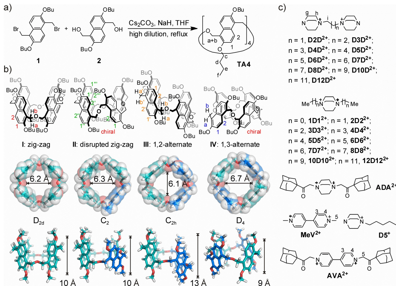
Fig. 1 (a) The synthetic procedure of per-butyl oxatub[4]arene ( TA4 ); (b) Chemical structures of four representative conformers of TA4 resulting from naphthalene flipping, and the top and side views of their models. In order to show the cavity in the most expanded forms, the models were obtained by forcing all the methylene protons in the linkers directed straightly outwards and the oxygen inwards. Numbering on the structures corresponds to the assignment of NMR signals. Conformers II and IV are chiral, but only one enantiomer is shown here. The lengths of the cavities are based on the distance between two oxygen atoms on the same naphthalene ring. The flipped naphthalene rings in conformations II , III , and IV relative to conformation I are colored in blue. Butyl groups in the models were abbreviated to methyl groups for viewing clarity; (c) Chemical structures of all the guests involved in this research; the counterions are \text{PF}_6^- .
