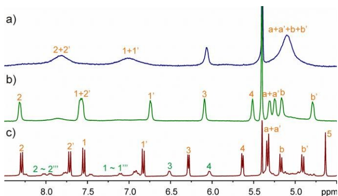
Fig. 5 Partial ^1\text{H} NMR spectra ( \text{CD}_2\text{Cl}_2:\text{CD}_3\text{CN}=1:1 , 2.0 mM) of the equimolar mixture of \text{TA}4 and \text{MeV}^{2+} at (a) 25 °C (400 MHz) or (b) -20 °C (600 MHz) and (c) \text{TA}4 and \text{AVA}^{2+} (400 MHz, 25 °C).
