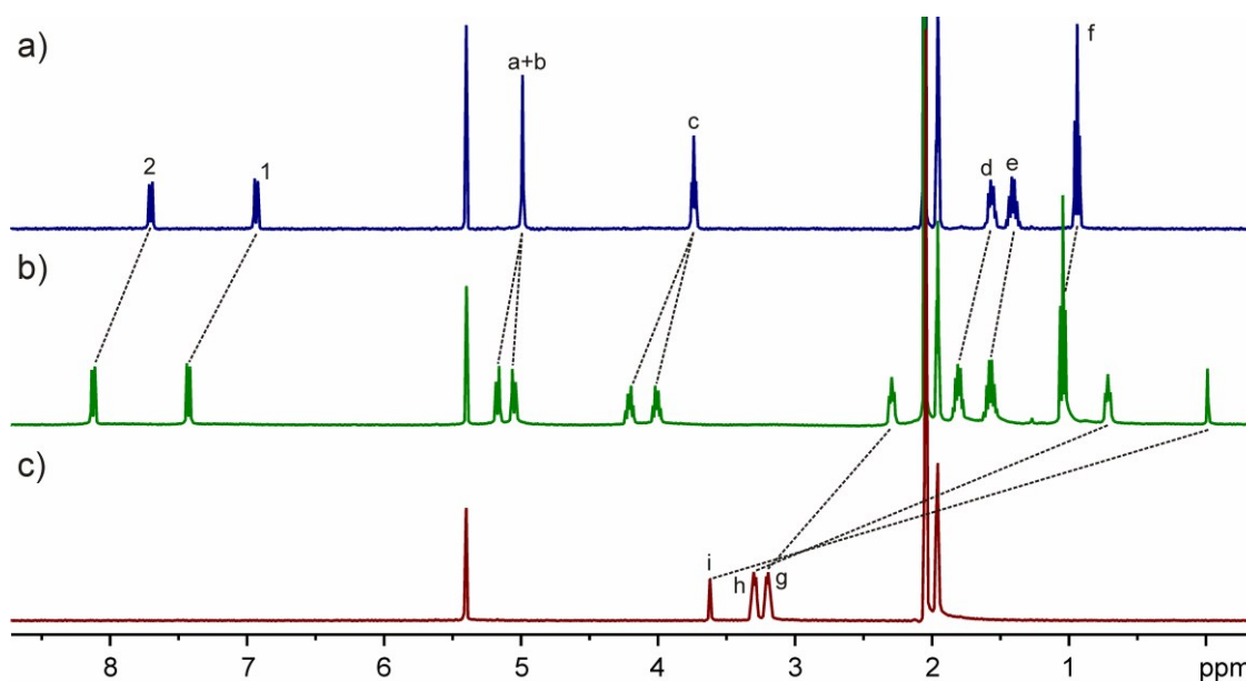
Fig. 2 Full ^1\text{H} NMR spectra (400 MHz, \text{CD}_2\text{Cl}_2:\text{CD}_3\text{CN}=1:1 , 2.0 mM, 25 ^\circ\text{C} ) of (a) TA4 , (c) D2D ^{2+} , and (b) their equimolar mixture. See Fig. 1 for signal assignments.
