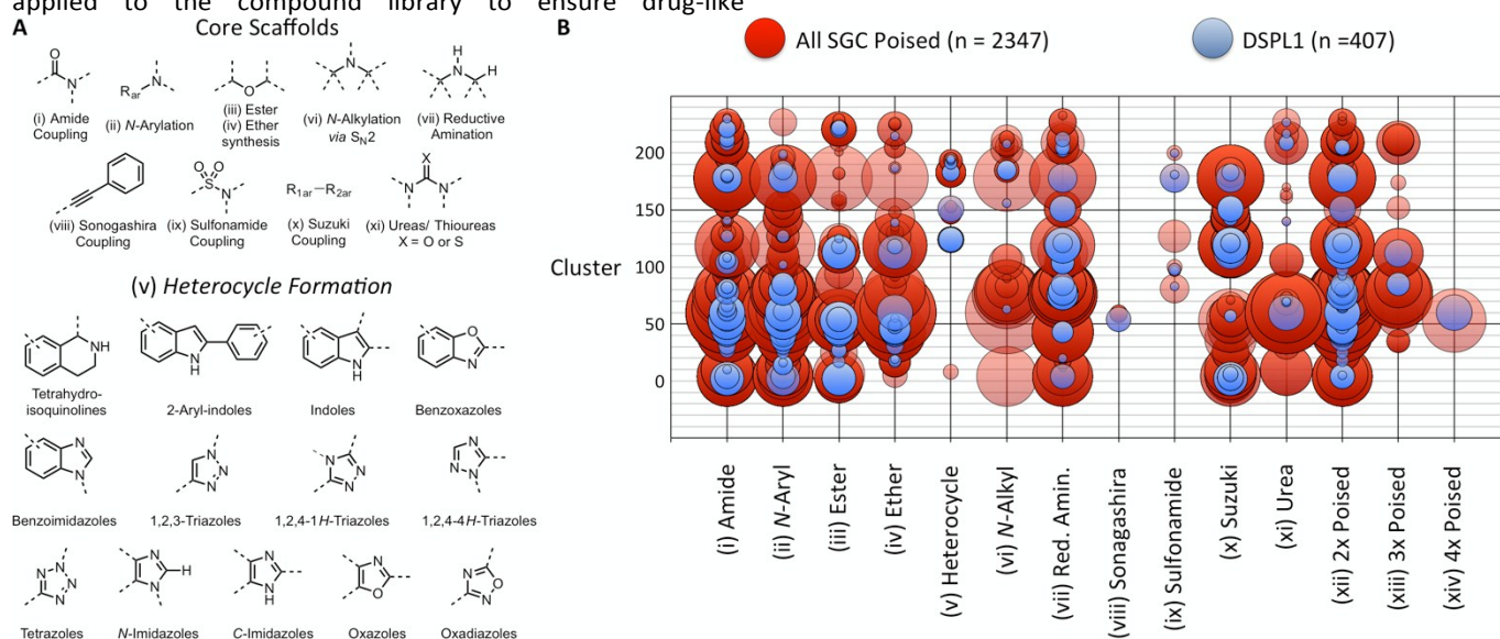
Fig 4 Design of DSPL1 (A) Scaffolds used to identify poised fragments. Core scaffolds based upon the most commonly used medicinal chemistry reactions as described by Roughley and Jordan. 33 Heterocycle scaffolds based on reactions described by Hartenfeller et al. 37 (B) Poised reaction motif vs cluster. Circle size represents the number of compounds in each group. 407 compounds for DSPL1 were selected from all SGC poised fragments based on diversity and poised reaction motif.
