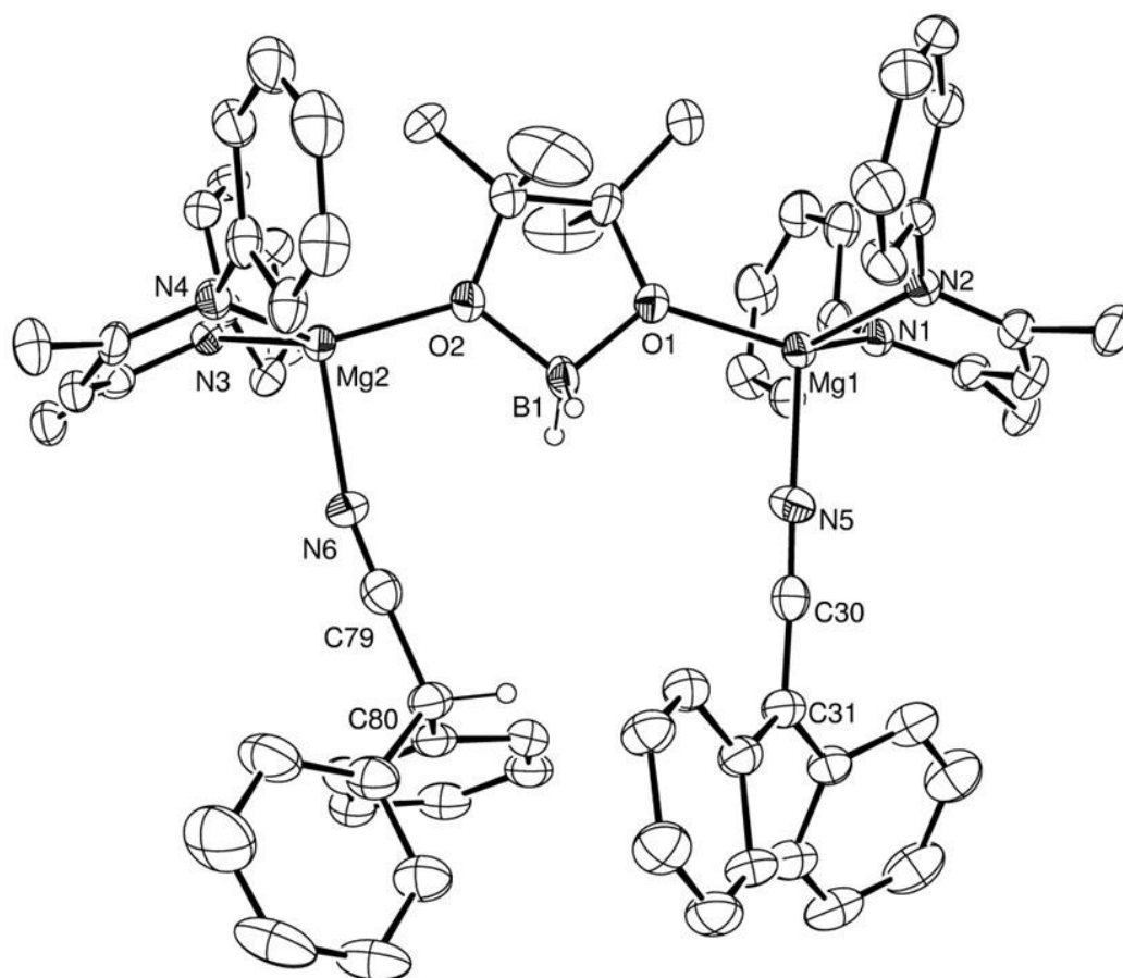
Figure 4: ORTEP representation of compound 5 (30% probability ellipsoids). Iso -propyl groups and hydrogen atoms other than that attached to C80 have been removed for clarity.
