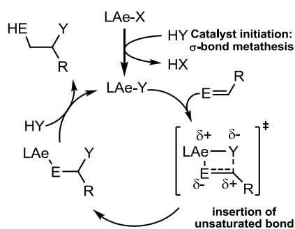
Scheme 1 Ae = Mg, Ca, Sr, Ba Y = R 2 N, R 2 P, RC≡C E = R 2 C, RN, O
