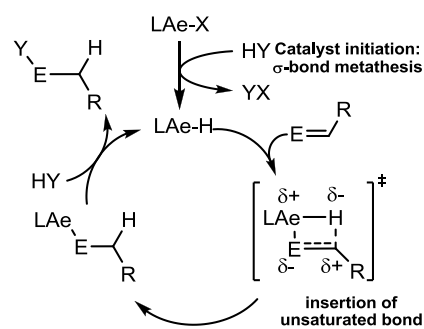
Scheme 2 Ae = Mg, Ca, Sr, Ba Y = R 3 Si, R 2 B, R 3 Sn E = R 2 C, RN, O
