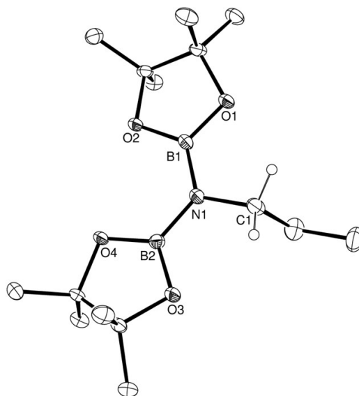
Figure 1: ORTEP representation of the structure of compound 1 (30% probability ellipsoids). Hydrogen atoms, except for those attached to the C1 methylene carbon centre, are omitted for clarity.
