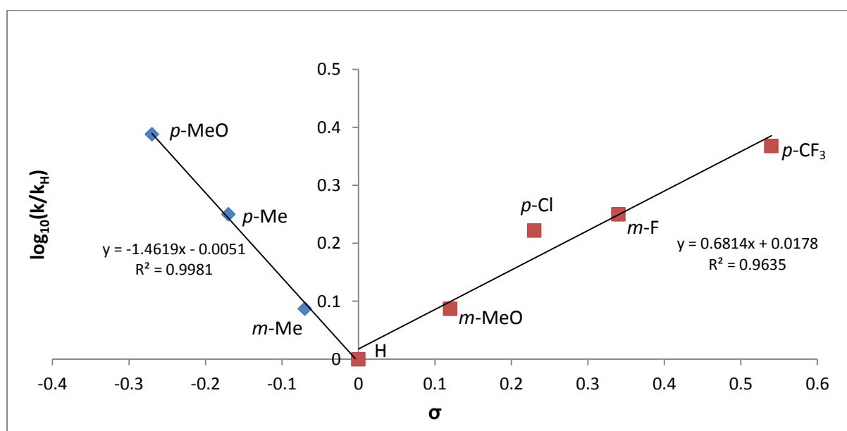
Figure 6: Hammett plot for dihydroboration of variously substituted aryl nitriles catalysed by V .
