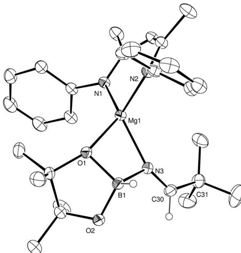
Figure 3: ORTEP representation of compound 4 (30% probability ellipsoids). Hydrogen atoms apart from those attached to B1 and C30 and iso -propyl groups are omitted for clarity.
