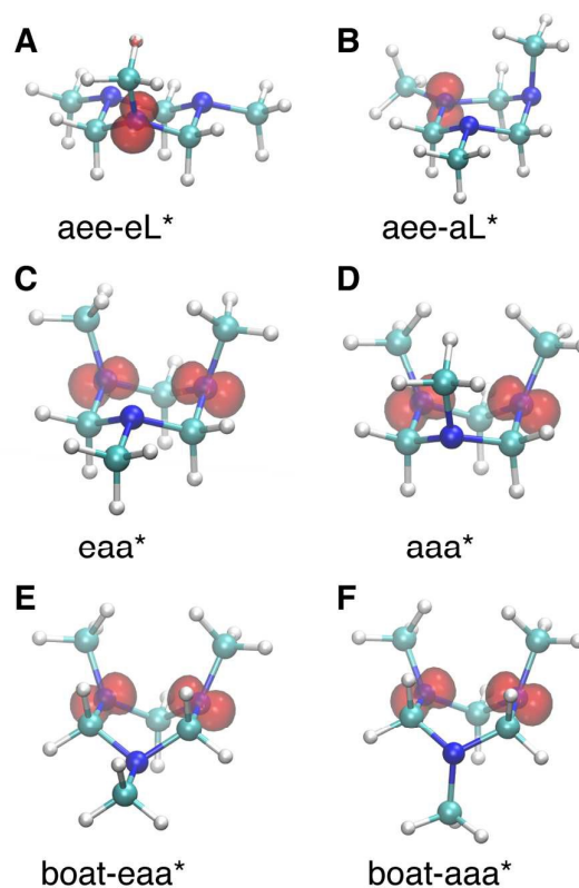
Fig. 6 The spin densities of molecular ion cores of Rydberg states for equilibrium cationic structures. (A) and (B) show the spin densities of the relaxed molecular ion cores reached by exciting the equatorial lone pair (eL) and the axial lone pair (aL) of the aee conformer, respectively. The charge is localized on the nitrogen atom where the electron is excited from. (C) – (F) are the spin densities with the most stable ion structures. The charge is delocalized between the two nitrogens with axial methyl groups. The rendered surface corresponds to a spin density of 0.2 Å -3 for (A) and (B) and 0.14 Å -3 for (C) – (F), about 10% of the maximum value.
