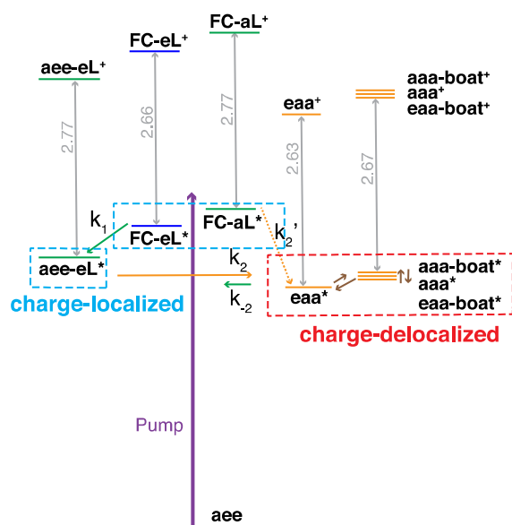
Fig. 7 Schematic summary of the structural dynamics of TMTAC after excitation. Species marked in the blue and red boxes designate charge-localized
