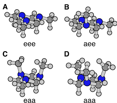
Fig. 3 The four chair conformers of TMTAC in the ground electronic state. The labels e and a refer to the equatorial and axial positions of the methyl groups, respectively.
