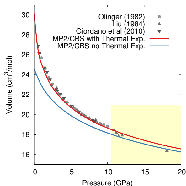
Fig. 5 Comparison of the experimental and predicted MP2/CBS pressure versus volume curves at 296 K, with and without quasiharmonic thermal expansion. Note that the drop in the experimental volumes above 10 GPa (shaded region) is believed to reflect a transition to phase III, 105 while the calculations presented are for phase I throughout.
