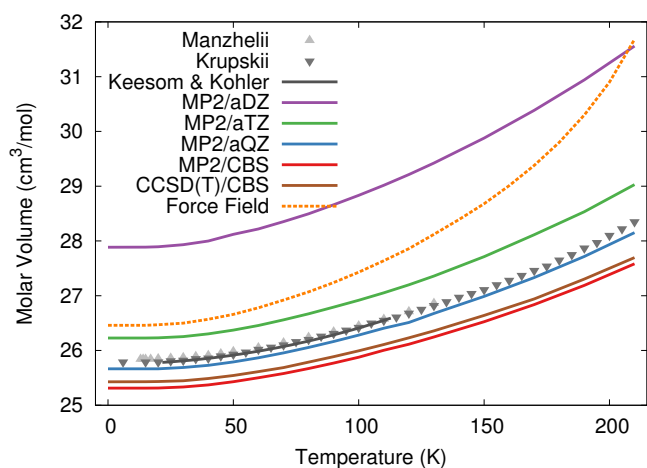
Fig. 1 Predicted thermal expansion of the \text{CO}_2(\text{s}) unit cell compared to the experimental values 88–91 in gray.
