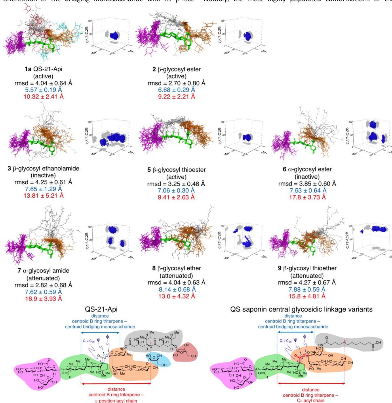
Fig. 3 Ensembles obtained from unrestrained 200 ns molecular dynamics simulations of QS-21-Api ( 1a ) and saponin variants 2 , 3 , and 5–9 . The rmsd (Å) for heavy atoms relative to average structure and three-dimensional plots of torsional angle distributions about the central glycosidic linker are shown. QS saponin structural domains are color-coded: branched trisaccharide (magenta), triterpene (green), linear trisaccharide (orange), acyl chain (gray), terminal sugars (QS-21 only: cyan, red). In the three-dimensional plots, torsional angle distributions are shown in blue and projections onto each plane are shown in gray. Active adjuvants exhibit distinctive and tightly-clustered torsional angle distributions about the central glycosidic linkage and comparatively shorter distances between the centroid of the triterpene B-ring and the centroid of the bridging monosaccharide (blue) as well as between the centroid of the triterpene B-ring and the acyl chain \epsilon -position (red). See Fig. S4–S8 for additional details.
