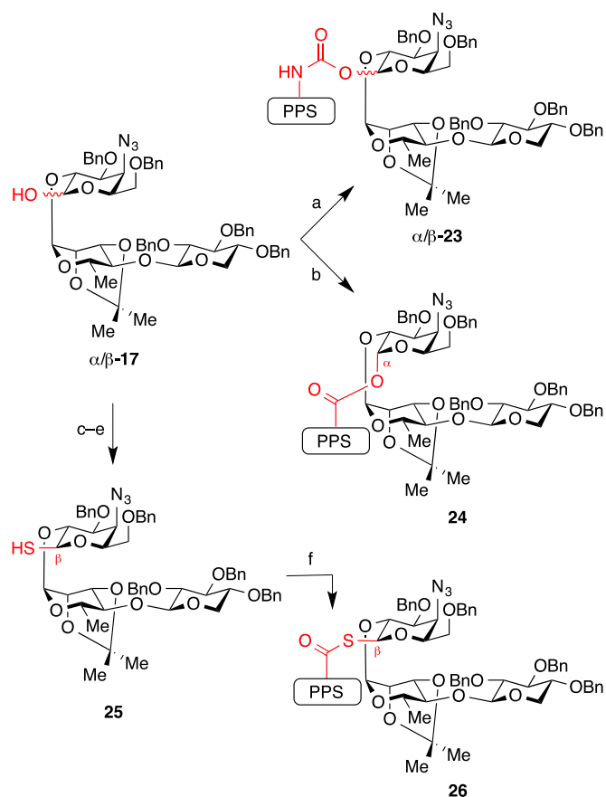
Scheme 3 Synthesis of glycosidic linkage variants using the glycosyl donor as a nucleophile. Reagents and Conditions: (a) NaH, then add 11 , THF, 79% combined yield of separable anomers (2:1 \beta/\alpha : 53% \beta - 23 , 26% \alpha - 23 ); (b) NaH, then add 12 , 1:1 THF/DMF, -20 °C, 70% (6:1 \alpha/\beta : 60% \alpha - 24 , 10% \beta - 24 ); (c) (COBr) 2 , DMF, TBP, CH 2 Cl 2 , 0 °C, 80%; (d) Cs 2 CO 3 , AcSH, 1:1 THF/DMF, 87% ( \beta only); (e) H 2 NNH 2 , DTT, 1:1 MeOH/THF, 94%; (f) 12 , NaH, THF, 0 °C, 87% ( \beta only). DTT = dithiothreitol.
