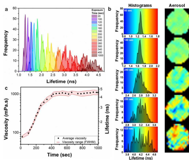
Fig. 5 Development of oleic acid droplet heterogeneity with exposure to ozone. a) Lifetime histograms recorded for an individual droplet ( 69.4 \mu\text{m} diameter) upon exposure to 377 ppm of ozone for 1000 sec. b) Selected histograms from (a) are shown next to their images, plotted against a rainbow colour hue of 1 ns width (same increment). c) The increasing average viscosity ( \bullet ) and a viscosity spread indicating heterogeneity (---) during ozone exposure; Gaussian fit of histograms in (a) provided peak centres as average viscosity values and the FWHM of histograms provided the spread.
