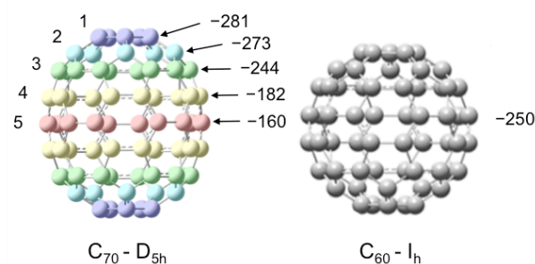
Fig. 6 Structures of C 70 -D 5h and C 60 -I h and LLIT 13 C DNP enhancements polarized at 0.33 T for different carbons of C 70 /C 6 D 6 /0.1M TEMPO system and the carbon of C 60 /C 6 D 6 /0.1M TEMPO system. Carbon atoms of C 70 are numbered from the apical to the equatorial positions. The relative standard deviation for A is about 15% (See Table S3).
