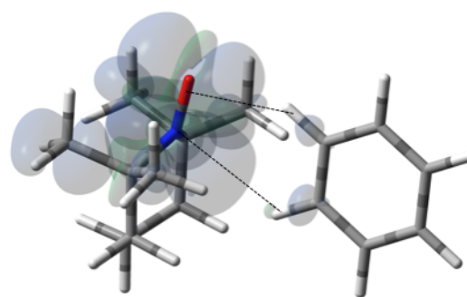
Fig. 11 The electronic spin density distribution of the largest ^{13}\text{C-H} HFC contributing orientation between benzene and TEMPO where two C-H moieties bite the TEMPO N-O group. Dashed lines are given as guides for intermolecular distances, which are 2.39 Å for O...H (of C-H moiety with closest approach to TEMPO oxygen) and 2.86 Å for N...H (of C-H with closest approach to TEMPO nitrogen).
