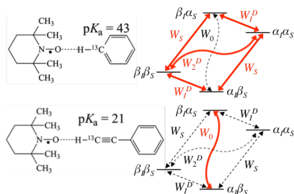
Fig. 1 Schematic diagram of energy level and transition probabilities for electron-nuclear ( 13 C) spin systems for benzene/TEMPO (above) and phenylacetylene/TEMPO (below). \alpha_S and \beta_S are the spin states of the unpaired nitroxide electron spin, and \alpha_I and \beta_I are for nuclear spins. W_S represents the electron relaxation; W_0 , W_1^D and W_2^D are zero, single and double quantum transition, respectively. W_0 is equal to the sum of W_0^{Sc} and W_0^D in eq. 3 and eq. 4, which are transition rates of scalar and dipolar relaxation, respectively. 13 C DNP enhancement of benzene is mainly due to dipolar relaxation, while scalar relaxation is the dominant mechanism for the \beta carbon of phenylacetylene.
