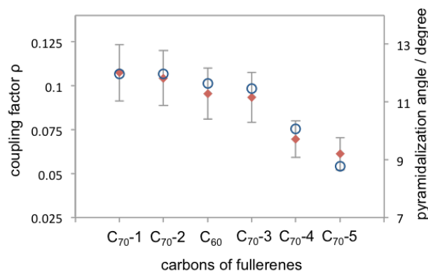
Fig. 8 Coupling factor derived from 13 C LLIT DNP absolute enhancements of the indicated carbons for C 70 -D 5h and C 60 are represented by red diamond; the pyramidalization angle of fullerene carbons for C 70 and C 60 95 are represented by blue circle.
