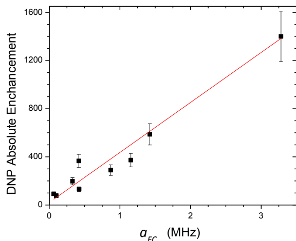
Fig. 18 Correlation between experimentally determined ^{13}\text{C} LLIT DNP scalar dominated enhancements and their calculated AFC (Boltzmann weighted DFT computed Fermi Contact hyperfine coupling constant) for the phenylacetylene/TEMPO, benzaldehyde/TEMPO, and nitrobenzene/TEMPO systems. After performing a linear regression with direct weighting of the DNP enhancement error, a line of best fit ( y = mx + b ) was determined having parameters m = 415 \pm 23 , b = 21 \pm 52 , and the goodness of the fit is computed as having an adjusted R^2 = 0.97 .
