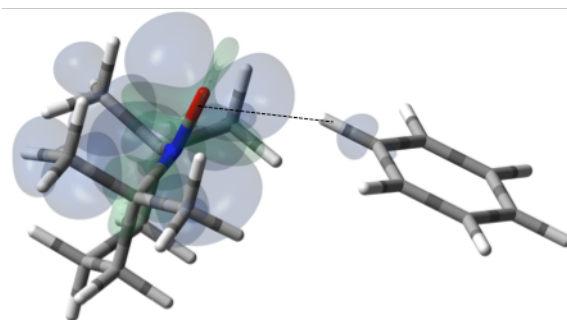
Fig. 12 The electronic spin density distribution of the second largest ^{13}\text{C-H} HFC contributing orientation between benzene and TEMPO where one C-H moiety points at N-O group. Dashed line is given as a guide for intermolecular distance, which is 2.30 Å between the oxygen atom of TEMPO and the hydrogen atom of benzene C-H moiety.
