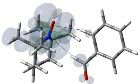
Fig. 15 The electronic spin density distribution for the largest ^{13}\text{C}\text{H}\text{O} - and ^{13}\text{C} - ortho HFC contributing orientation between benzaldehyde and TEMPO where the aldehyde and ortho C-H moieties bite the N-O group. Dashed lines are given as guides for intermolecular distances, which are 2.39 Å for O---H (of ortho C-H) and 2.46 Å for N---H (of aldehyde C-H).
