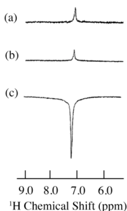
Fig. 5 ^1H spectra of 9% benzene/0.001M TEMPO dissolved in SF CO_2 at 4.7 T. (a) Static ^1H NMR ( S/N = 20 ), (b) flow ^1H NMR ( S/N = 17 ) and (c) flow ^1H DNP ( S/N = 124 ). Total flow of SF CO_2 was 1.1 mL/min. SF CO_2 conditions: d = 0.805 g/mL, SFC oven temperature 40 °C, P = 165 atm. All Spectra were collected at 32 scans.
