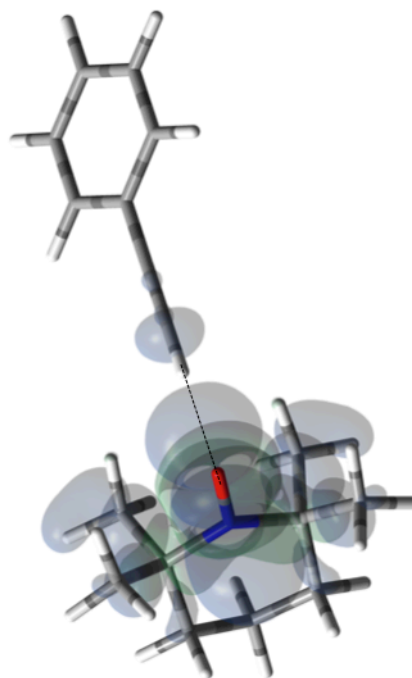
Fig. 17 The electronic spin density distribution of the largest ^{13}\text{C} - \beta HFC contributing orientation between phenylacetylene and TEMPO where the alkyne points at N-O group. Dashed line is given as guide for intermolecular distance, which is 2.03 Å between oxygen atom of TEMPO and the hydrogen atom of acetylene group of phenylacetylene
