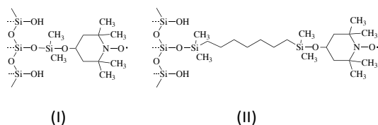
Fig. 3 Immobilized nitroxide material I (left) and II (right) used in SLIT 1 H DNP in normal liquids and SF CO 2 .
