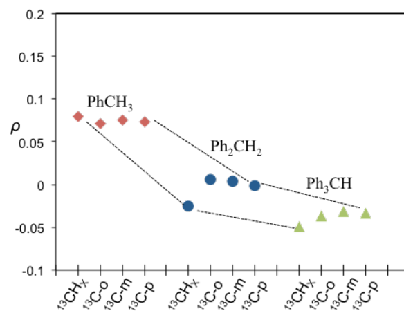
Fig. 9 Coupling factor derived from ^{13}\text{C} LLIT DNP absolute enhancements of the indicated carbon (i.e. ^{13}\text{CH}_X , X=1-3 , ^{13}\text{C-ortho} , ^{13}\text{C-meta} , and ^{13}\text{C-para} ) for the series of toluene (red diamond), diphenylmethane (blue circle), and triphenylmethane (green triangle) ( \text{Ph}_Y\text{CH}_X , X=1-3 , Y=4-X ). 66 Dashed lines illustrate motif trends for different molecules. The relative standard deviation for \rho is about 15%.
