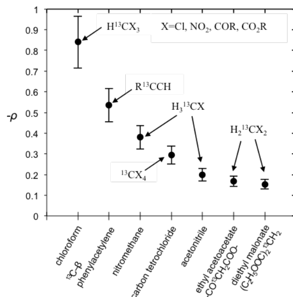
Fig. 10 Coupling factor (negative) derived from scalar dominant ^{13}\text{C} LLIT DNP absolute enhancements of small molecules. The relative standard deviation for \rho is about 15%.
