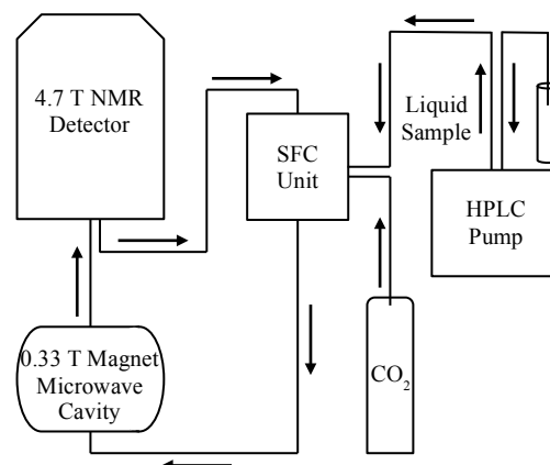
Fig. 4 Schematic drawing of apparatus for continuous-flow HPLC-DNP-NMR coupled with SF CO 2 (adapted from Ref.43, with the original Figure shown in SI).
