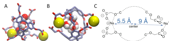
Figure 8. \text{Na}^+ counter ions (yellow) near the m3n3 cryptophane molecule in the absence of Xe ( \lambda = 1 ). A) Top view. B) Side view ( 90^\circ rotation of configuration in A). C) Schematic illustration of counter ion coordination by the side chains.
