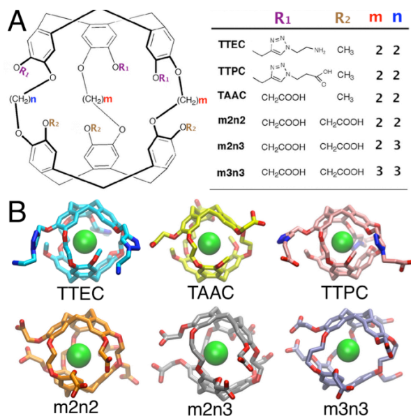
Figure 1. A) The structures of six water-soluble cryptophanes. B) Renderings of cryptophane molecules with Xe bound.
