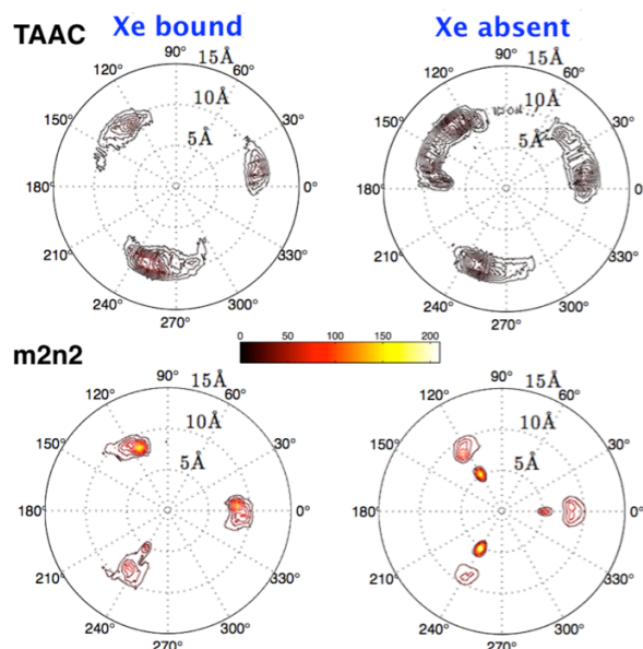
Figure 10. Polar contours for distribution of counter ions. The left and right columns are the polar distributions of counter ions when \lambda = 0 and \lambda = 1 , respectively. The origin is set at the center of mass of the 36 aromatic carbon atoms of the cryptophane; the x-y plane is perpendicular to the vector connecting the two centers of mass of the top and bottom caps, and the x axis is the projection of the vector connecting the origin and the average position of two phenol oxygen atoms on the same linker. On the contour plot, the radial coordinate r is the distance between the origin and a counter ion; \theta is the angle between the x axis and the projection of r on the x-y plane. Color scale bar is shown above for g(r, \theta) .
