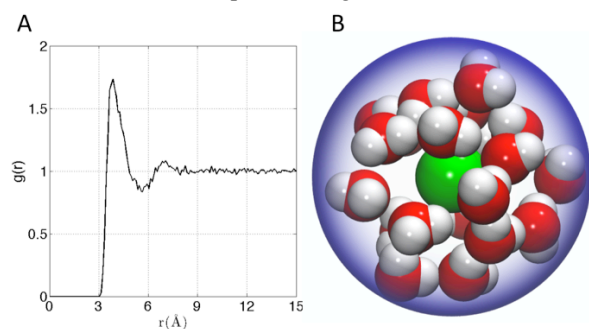
Figure 6. A) Water radial distribution function g(r) about Xe in water, where r is Xe-O distance. B) Sampled configuration depicting first solvation shell (waters within 6 \text{ \AA} ) of Xe in water.
