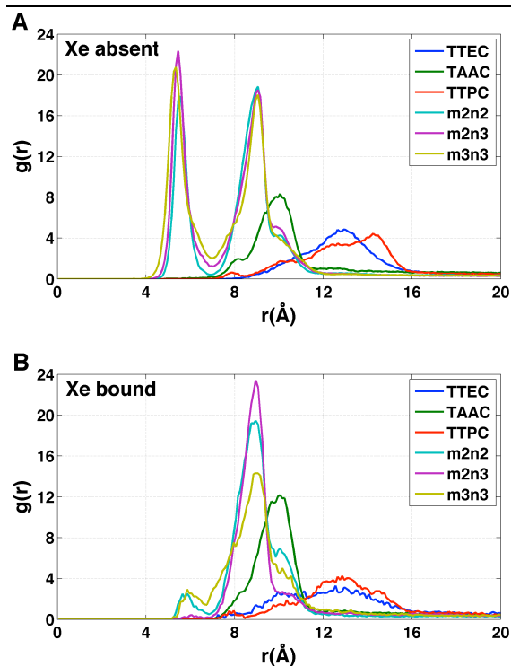
Figure 9. The radial distribution g(r) of counter ions relative to the center of mass of the cryptophane molecule. A) Xe atom is absent ( \lambda = 1 ). B) Xe atom is present within the cryptophane ( \lambda = 0 ).
