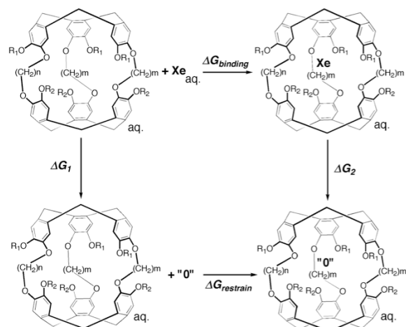
Figure 2. Thermodynamic cycle of double decoupling method. All simulations are performed in an aqueous environment. The state “0” indicates the complete decoupling of Xe atom from its environment when potential energy terms involving the Xe atom vanish.
