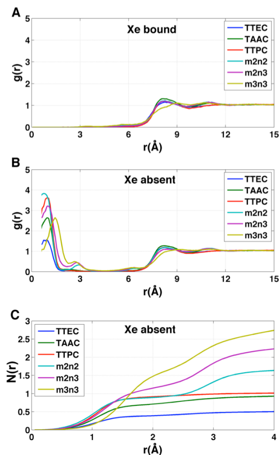
Figure 5. Distribution of water molecules in cryptophane interior. The distance r is measured between the cryptophane center of mass and a water oxygen nucleus. A) Radial distribution function g(r) for water when Xe is present in the interior ( \lambda = 0 ). B) Radial distribution function g(r) for water when Xe is absent from the interior ( \lambda = 1 ). C) Average number of water molecules N(r) within a distance r from the cryptophane center of mass in the absence of Xe. Curves are obtained from integrating the corresponding g(r) .
