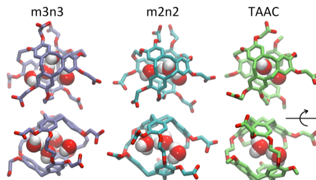
Figure 4. Configurations with water molecules inside cryptophanes m3n3 , m2n2 and TAAC. In the lower row, each configuration is rotated 90^\circ .
