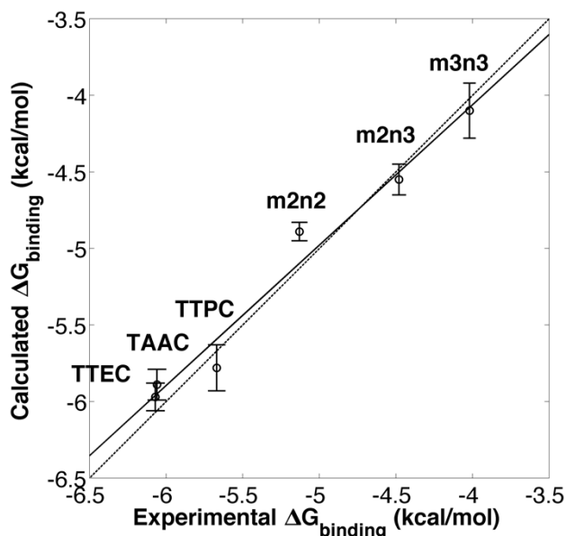
Figure 3. Experimental 6, 20, 21, 24 and calculated free energies of Xe binding. The solid line is a linear least squares fit. The dotted line corresponds to equality of the experimental and calculated values of \Delta G .
