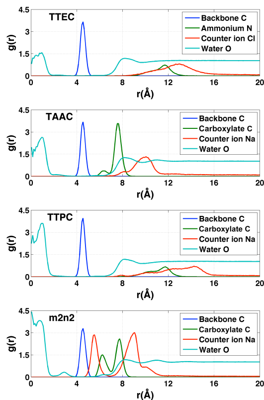
Figure 11. Radial distribution functions of atoms associated with simulations of the cryptophanes TTEC, TAAC, TTPC, and m2n2 in the absence of Xe. In each case, r is the distance of the indicated atom type to the center of mass of the cryptophane. Blue (backbone): the aromatic carbon atoms of the cryptophane. Green (ionizable groups in the side chains): for TTEC, the ammonium nitrogen atom N; for TAAC, TTPC and m2n2, the central carbon of the carboxylate group. Red (counter ions): \text{Cl}^- for TTEC and \text{Na}^+ for TAAC, TTPC, and m2n2. Cyan (water): the oxygen atoms of water molecules. The blue, green and red distribution functions have been rescaled by dividing by 100, 25 and 6, respectively.
