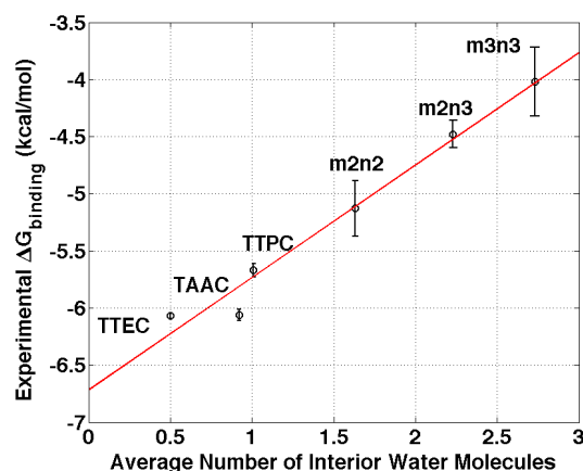
Figure 13. Correlation between the average number of interior water molecules and experimental free energies of Xe binding. 6, 20, 21, 24 The red solid line is a linear least squares fit. The radius cutoff for identifying interior waters was set at 4 Å relative to the center of mass of the 6 aromatic rings of cryptophane molecules.
