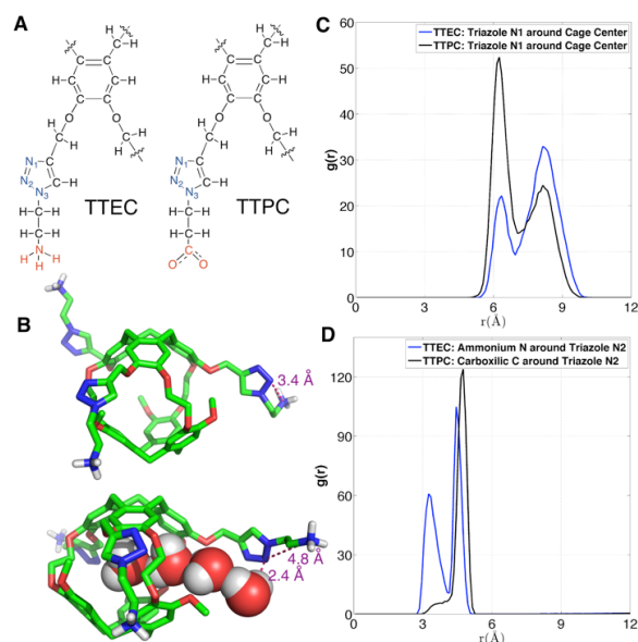
Figure 12. Triazole side chains and solvation of TTEC and TTPC. A) Structures of the triazole side chains of TTEC and TTPC. The triazole N atoms are marked blue, and their different terminal groups are marked red. B) Two configurations of triazole side chains in TTEC. C) Radial distribution function of triazole \text{N}_1 atoms relative to the mass-weighted cryptophane centers in TTEC (blue) and TTPC (black). D) Radial distribution functions of ammonium N atoms (TTEC, blue) and carboxylate C atoms (TTPC, black) relative to the triazole \text{N}_2 atoms.
