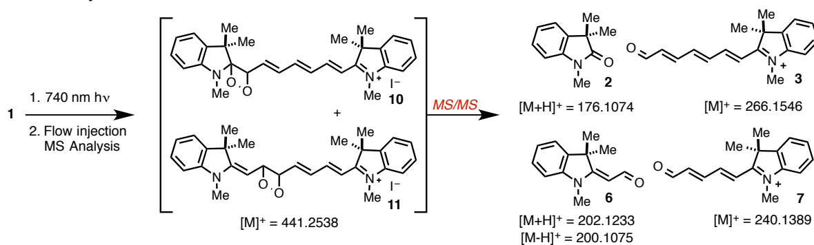
Figure 1: (A) Photoproducts observed by HRMS upon 740 nm light irradiation of 1 and (B) MS/MS [1+O_2] adducts.
