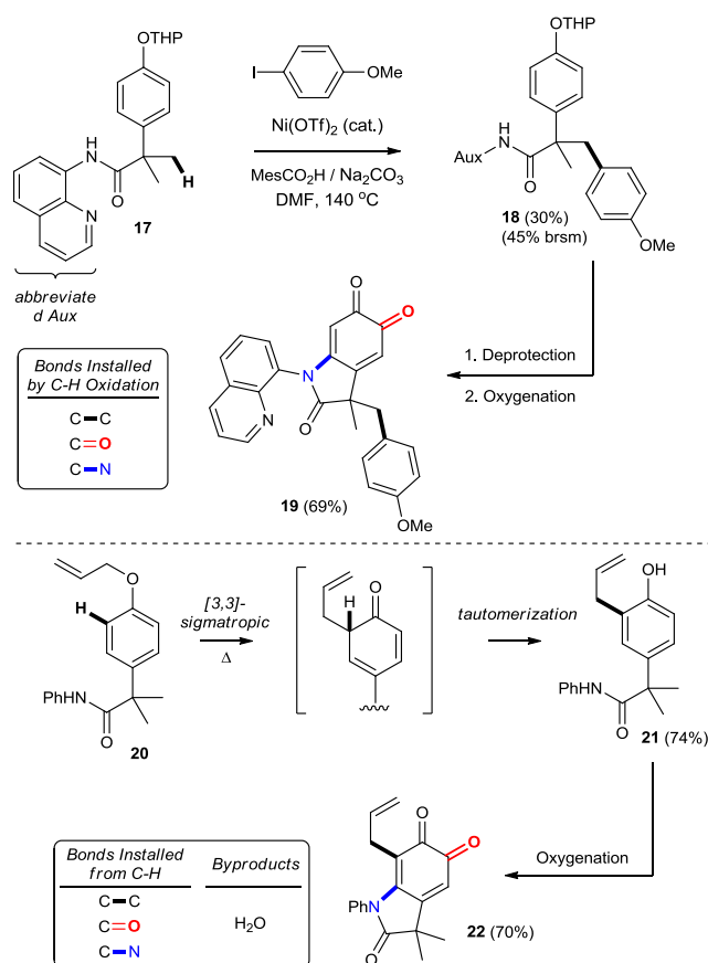
Scheme 8. Product diversification by orthogonal C-H functionalization. See Supporting Information for detailed experimental procedures.
