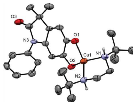
Figure 2. ORTEP at 50% ellipsoid probability of one molecule of SQ3 , a cation, in the X-ray structure of ( SQ3 ) 2 (SbF 6 ) 2 ·2.5 CH 2 Cl 2 . H atoms except those on N1 and N2 are omitted for clarity. Selected bond lengths (Å): Cu-N1 1.992(5), Cu-N2 1.994(4), Cu-O1 1.955(4), Cu-O2 1.946(4), C1-O1 1.284(6), C2-O2 1.291(6). Dihedral angle between N1Cu1N2 and O1Cu1O2 planes: 50.34°.
