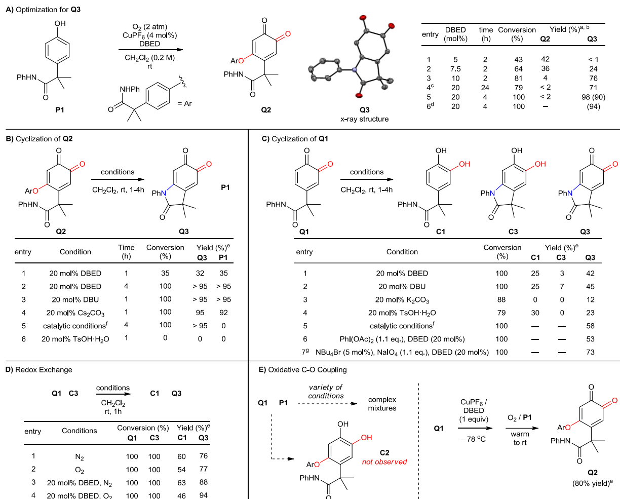
Scheme 3. Optimization of reaction conditions and control experiments. [a] Reactions performed with 0.5 mmol of P1 . Work-up: 10% aqueous NaHSO 4 . [b] Product yield determined by 1 H-NMR using hexamethylbenzene as an internal standard. Isolated yield reported in parenthesis. [c] Reaction performed under open-flask conditions. [d] Reaction performed using 5 g of P1 . [e] Reactions were performed with 0.1 mmol of starting material, and analyzed by 1 H-NMR following acidic work-up using hexamethylbenzene as an internal standard. [f] Catalytic conditions: [Cu(MeCN) 4 ](PF 6 ) (4 mol%), DBED (20 mol%), O 2 (2 atm). [g] Reaction performed in a biphasic mixture of CH 2 Cl 2 (10 mL) and water (2 mL).
