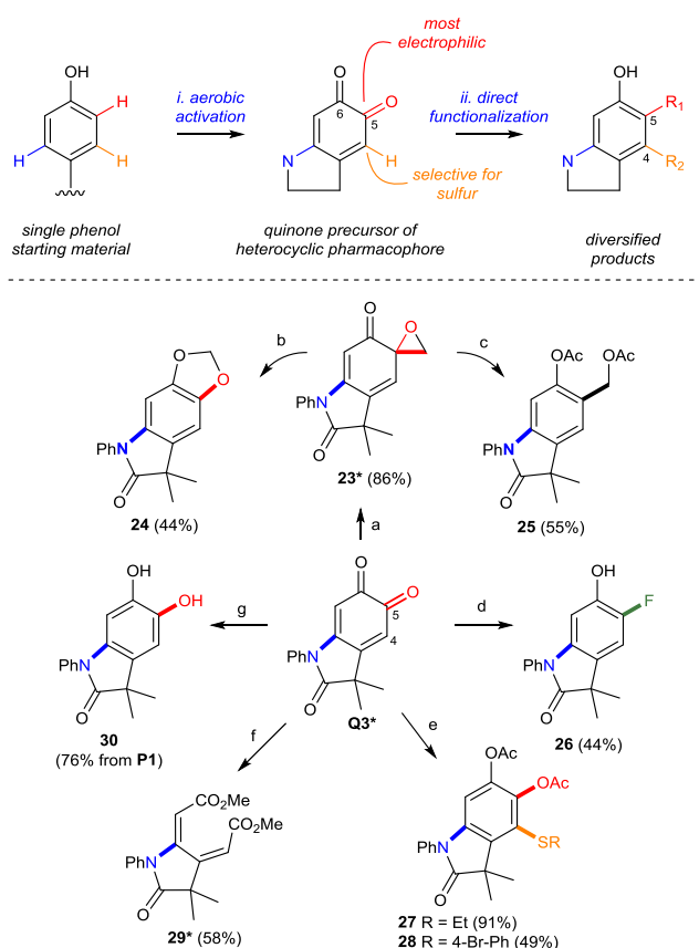
Scheme 9. Synthetic Diversification of Q3 . Yields in parenthesis are based on the amount of Q3 without other notification. a) [\text{Cu}(\text{MeCN})_4](\text{PF}_6) , \text{CH}_2\text{N}_2 , THF. b) TBSCl, \text{NEt}_3 , PhMe. c) \text{CeCl}_3 , \text{NaBH}_4 , then \text{Ac}_2\text{O} . d) Deoxofluor ® , \text{CHCl}_3 , then \text{NaBH}_4 , DBU, MeOH. e) R-SH, DIPEA, \text{CH}_2\text{Cl}_2 , then \text{Ac}_2\text{O} . f) \text{Pb}(\text{OAc})_4 , PhMe/MeOH. g) \text{Na}_2\text{S}_2\text{O}_4 workup. *Characterized by X-ray crystallography. See the supporting information for details of the crystallographic characterization and experimental procedures.
