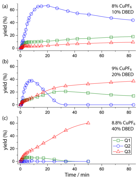
Figure 3. Yields of Q1 (green squares), Q2 (blue circles), and Q3 (red triangles) during the reaction under three sets of conditions, deduced by fitting UV-vis spectra at various time points (See Figs S7–S9 for full data including SQ1–3 ). Conditions: \text{CH}_2\text{Cl}_2 , 25 °C \text{CH}_2\text{Cl}_2 , \text{O}_2 (1 atm), 15.67 mM P1 and (a) 8% \text{CuPF}_6 , 10% DBED; (b) 9% \text{CuPF}_6 , 20% DBED (as in Fig. 1); (c) 8.8% \text{CuPF}_6 , 40% DBED. The y-axis is scaled to the maximum concentration of each species, i.e. [\text{Q1}]_{\text{max}} = [\text{Q3}]_{\text{max}} = [\text{P1}]_0 and [\text{Q2}]_{\text{max}} = 0.5 [\text{P1}]_0 . Thus each point in the graph gives the yield of each species.
