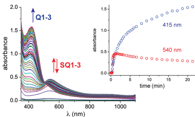
Figure 1. In-situ UV-vis spectroscopic monitoring under catalytic conditions: CH 2 Cl 2 , 25 °C, 15.67 mM P1 , 9% CuPF 6 , 20% DBED, O 2 (2 atm), 1.0 mm pathlength. Inset: absorbance profile at 415 and 540 nm. To ensure homogeneous mixtures of P1 , UV-vis experiments were conducted at a low concentration of P1 . To improve the rate of conversion, the Cu loading was increased to 8-9%.
