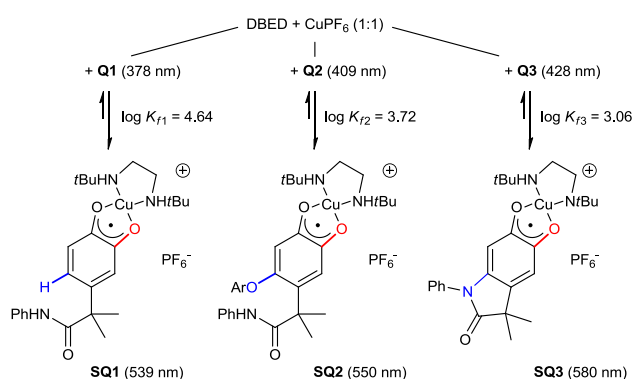
Scheme 4. Independent synthesis of SQ1-3 by coordination and electron-transfer of DBED-Cu(I) to Q1-3 , with binding constants and main spectral features. Details in Figures S3-S6.
