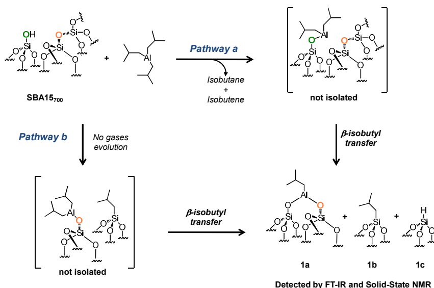
Scheme 2. Reaction of TIBA (1M/hexane) with single silanol (pathway a) and strained siloxane bridges (pathway b) of SBA 15700 at room temperature.
