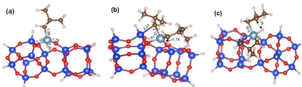
Fig. 7. DFT optimized geometry of (a) the Al-H intermediate b3'' , (b) of the transition states b2-b3 and b2-b3'' , for alkyl transfer to the silica, and (c) the \beta -H elimination to the Al. Distances are in Å.
