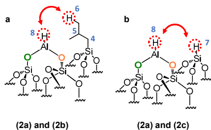
Scheme 8. Representation of the close proximity of (a) aluminum hydride 2a and silicon isobutyl 2b , (b) aluminum hydride 2a and silicon hydride 2c .
