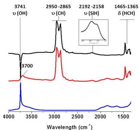
Fig. 1. IR spectra of (i) SBA15 700 (blue), (ii) SBA15 700 after reaction with 1 equiv. of TIBA/ \equiv\text{SiOH} (red) and (ii)-(i) subtraction of spectra (ii) and (i) (black).
