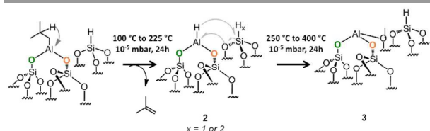
Scheme 4. Formation of Aluminum hydride through a thermal treatment (100 °C to 400 °C) under 10^{-5} mbar for 20 h of 1 .
