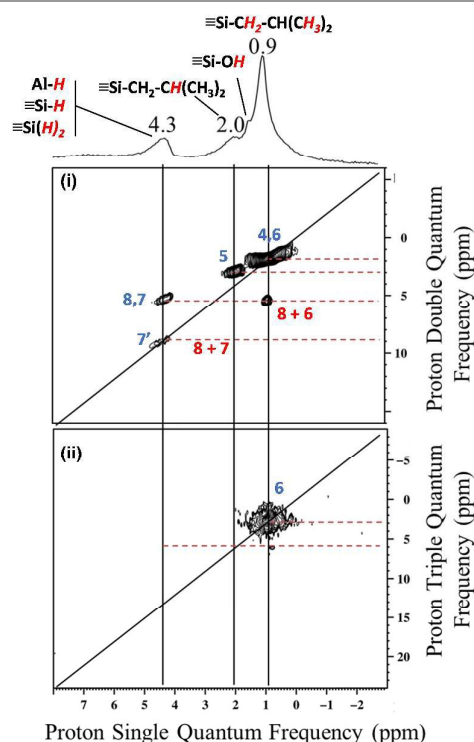
Fig. 9. (i) DQ rotor-synchronized 2D 1 H MAS NMR spectrum of 2 . (ii) 1 H TQ MAS spectra of 2 (7' is ascribed for \text{SiH}_2 )
