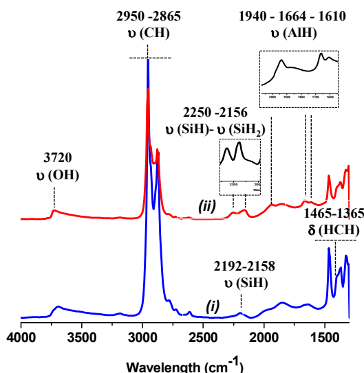
Fig. 8. (i) IR spectra of 1 , (ii) after thermal treatment at 225 °C for 24 h. Inlet subtraction (ii)-(i) in the corresponding area of silicon and aluminum hydride, respectively.
