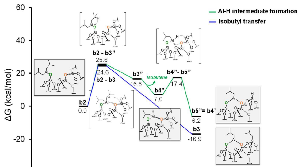
Fig. 6. Energy profile for the reactivity of monopodal [\equiv\text{SiO-Al-CH}_2\text{CH}(\text{CH}_3)_2]_2 with siloxane bridges, (\equiv\text{Si-O-Si}\equiv) . Alkyl transfer versus two step H transfer.
