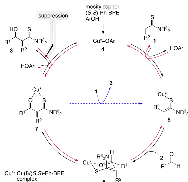
Fig 1 Proposed catalytic cycle. Black arrows represent the forward pathway of the desired aldol reaction. Blue arrows represent a bypass route in which Cu(I)-aldolate 7 functioned as a catalyst. Red arrows represent retro-aldol pathways.
