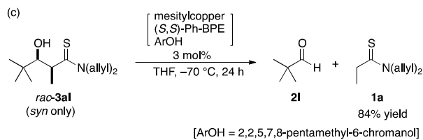
Scheme 4 Forward and retro reaction using \alpha -fully substituted aldehyde 2l .
