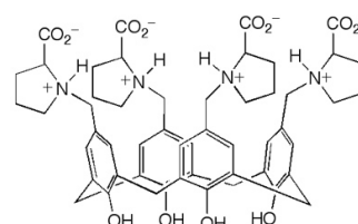
Figure 1. Proline-functionalised calix[4]arene, 1 , the low molecular weight hydrogelator used in this study.
