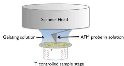
Figure 2. Schematic of the experimental set up used for in situ variable temperature scanning probe microscopy of gel formation.
