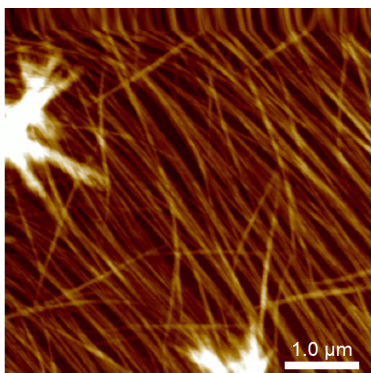
Figure 4. Atomic force micrograph of a 1 /MgCl 2 hydrogel smeared and imaged ex situ on a mica substrate, showing alignment of the fibres presumed to be induced by the sample preparation.
