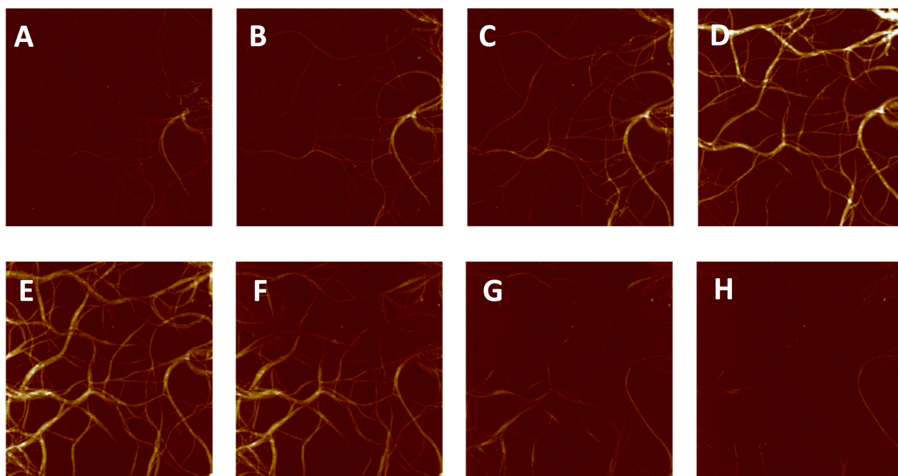
Figure 3. In situ images and cross sectional analysis of fibres formed by an aqueous mixture of 1 (25 mM) and \text{MgCl}_2 (20 mM) with changing temperature. All cross sections were taken as an average over a length of 250nm along the fibre. The height scale is 0 to 30 nm, and scan size is 5 \mu\text{m} , in all images; 4.4 min/image. The full set of images are provided in Figure S1.
