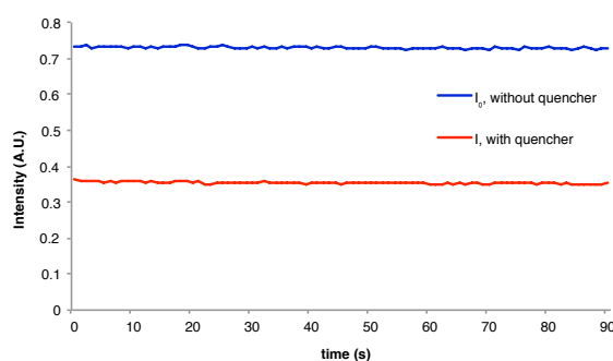
Figure 3. Phosphorescence intensity during reaction.
