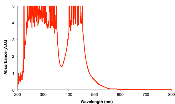
Figure 1. UV-vis absorption spectrum for \text{Ru}(\text{bpz})_3(\text{BArF})_2 at 4 \times 10^{-4} M in \text{CH}_2\text{Cl}_2 .
