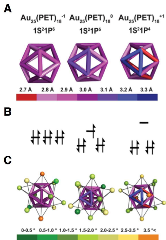
Figure 3. A) A heat map of the edge bond length of the \text{Au}_{13} cores of \text{Au}_{25}(\text{SR})_{18}^{-1/0/+1} . B) An energy level diagram of the P orbitals. C) A heat map of the distortion away from face capping the Au(I) as judged by angles to the core.
