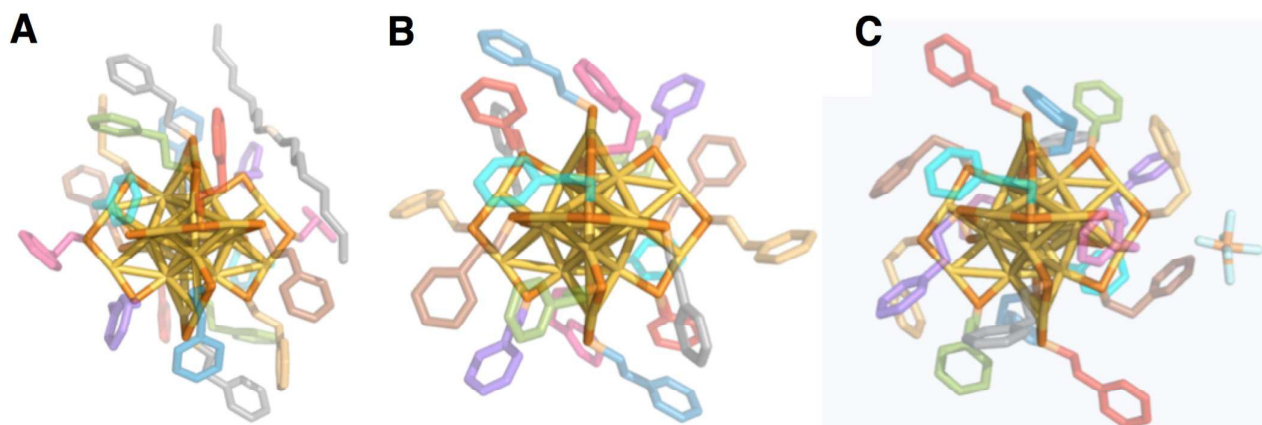
Figure 1. The crystal structures of \text{Au}_{25}(\text{PET})_{18} in the -1 (A), 0 (B), and +1 (C) charge states are shown above. Gold is in yellow, and sulfur is in orange. Crystallographically independent PET ligands are shown in unique color (see Table 1).
