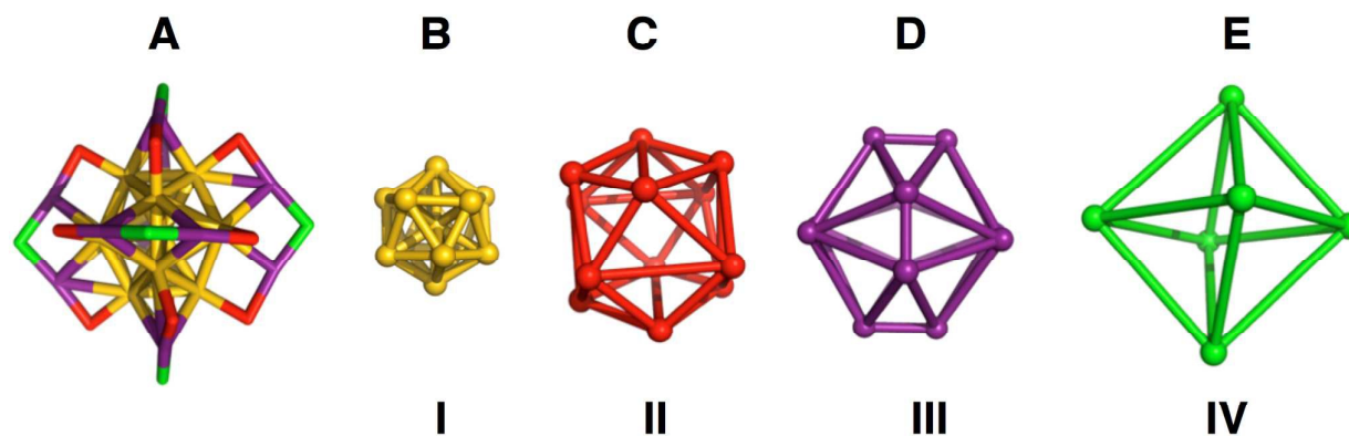
Figure 2. A) Structures of the inorganic core and semirings of [\text{Au}_{25}\text{PET}_{18}]^{+1}[\text{PF}_6]^{-1} , with each color highlighting a different symmetry for sulfur or gold. In B-E) the shape in which each unique atom makes is displayed, B) is a gold icosahedron, C) a distorted sulfur icosahedron, D) a dodecahedron missing 8 vertices that form the vertices of an inscribed cube, each vertex shown corresponds to an Au(I) atom and E) is a sulfur octahedron.
