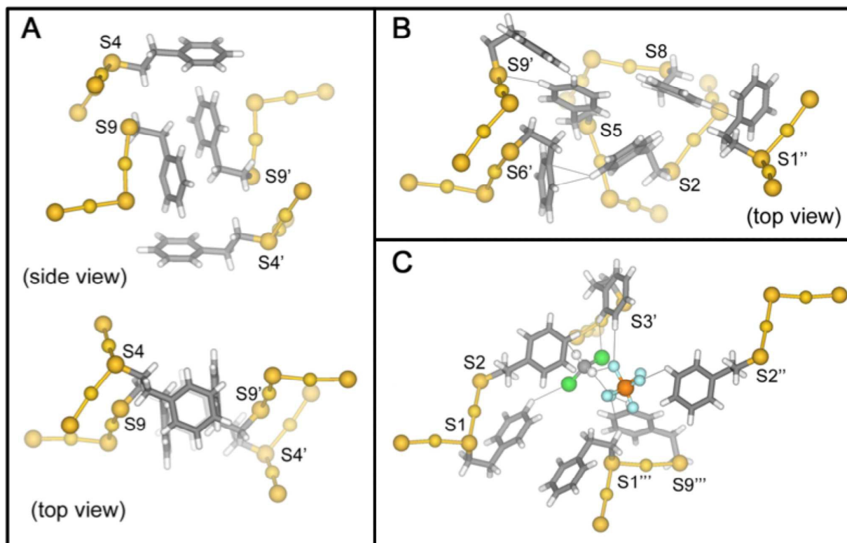
Figure 7. The π-stacking squares formed by PET4 and PET9 of adjacent clusters are shown in panel A. The extended π-interaction network of PET1, PET2, and PET8 with PET5, PET6 and PET9 of an adjacent cluster are shown in panel B. The ligands involved in phenyl-halogen and phenyl-solvent interactions important for crystal packing are shown in figure C. Ligands of neighboring clusters are denoted by an apostrophe.
