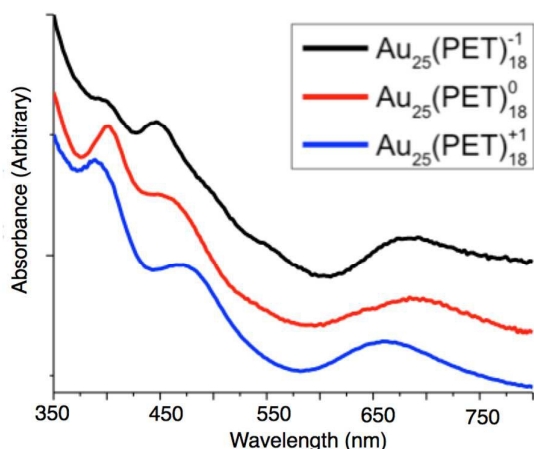
Figure 5. The linear absorption spectra of \text{Au}_{25}(\text{SR})_{18}^{-1/0/+1} . The spectra are normalized and offset for clarity.
