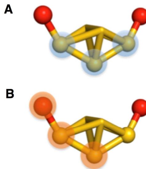
Figure 4. Depicted above is the two planes used to measure the dihedral angles of the semi-rings. A shows the plane defined by the core and B shows the plane defined by the semi-ring. The plane on B is changed to incorporate the appropriate atom in the semi-ring and is measured on both sides.
