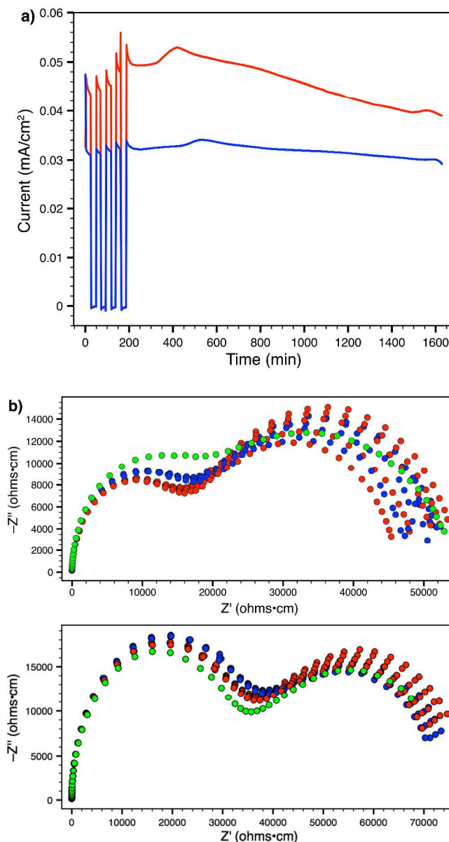
Fig. 7. (a) Current response from 300 mV applied potential to 14 (red) and 19 (blue) in a symmetric lithium metal cell. (b) AC impedance spectra collected during 24-hour operation of \text{Li(s)}|\text{electrolyte}|\text{Li(s)} symmetric cells. Top: polymer 14 . Bottom: polymer 19 . Red data represents impedance spectra taken without constant applied voltage. Blue data represents Blue data represents spectra taken with 300 mV applied voltage. Green data represents the final spectrum taken after the experiment.
