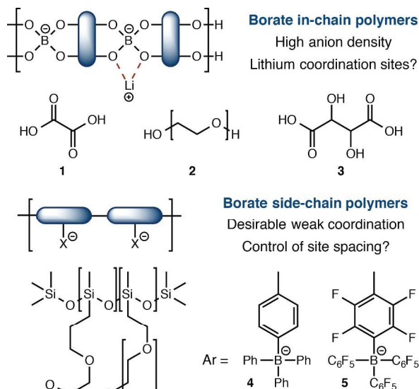
Fig. 1. Current approaches and limitations to borate containing single-ion polymer electrolytes.
