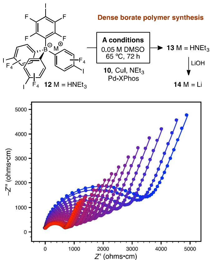
Scheme 2. Synthetic approach to perfluorinated polymer 14 and variable-temperature ac impedance spectra taken from 300 K (blue circles) to 373 K (red circles) in 5 K intervals from 303 K on. Lines represent fit to an equivalent circuit diagram shown in the Supporting Information.
