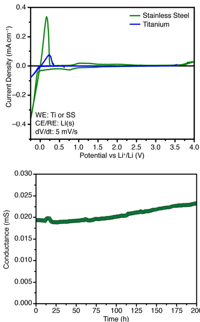
Fig. 5. Cyclic voltammograms of electrolyte 14 using titanium and stainless steel working electrodes at 90 °C (top), and time dependence of total conductance measured at room temperature in a symmetric Li(s)|electrolyte|Li(s) cell (bottom).
