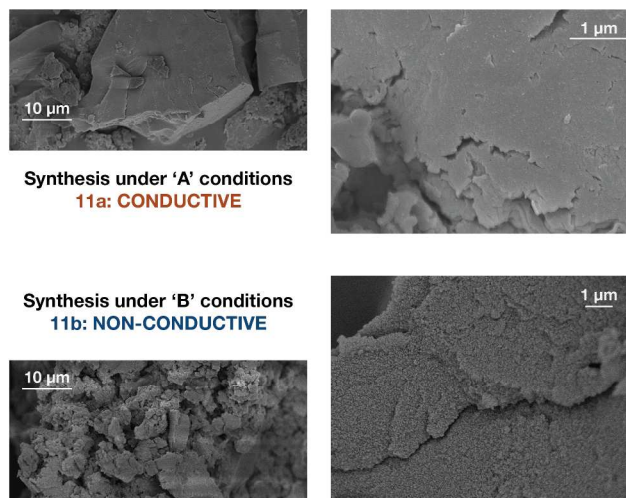
Fig 4. Scanning electron micrographs of borate polymers produced in DMSO ( 11a above) and DMF ( 11b below).
