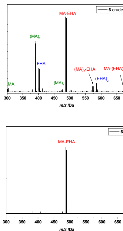
Figure 5. ESI-MS spectra of I-MA-EHA-Br 6 , before and after purification. For synthesis of 6 , MA and EHA were inserted subsequently, without intermediate purification, so both homo-oligomers as well as MA-EHA block-co-oligomers are observed in the crude product.
