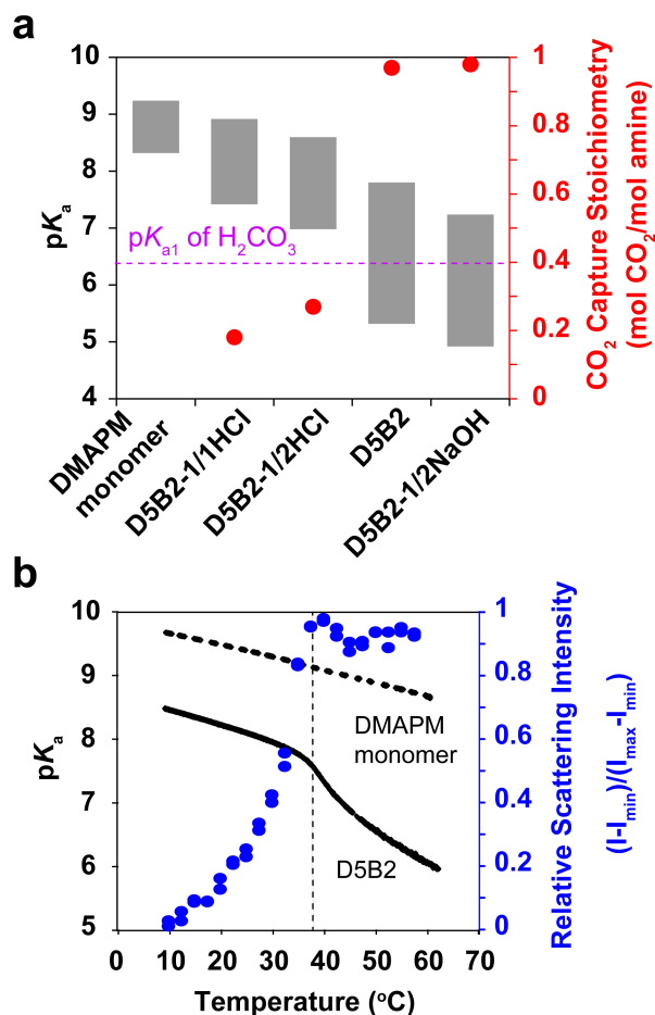
Fig. 1 (a) pK_a values (left Y-axis) of D5B2-1/1HCl, D5B2-1/2HCl, D5B2, D5B2-1/2NaOH and the monomer DMAPM at 75 °C (bottom of bar) and 30 °C (top of bar), and the reversible CO_2 capture stoichiometries (right Y axis, red dot) of the GP films in the temperature range 30–75 °C. (b) pK_a shift (left Y-axis) of D5B2 (black solid line) and the monomer DMAPM (black dashed line) during the heating process, and the temperature dependent relative scattering intensity (right Y-axis, blue dot) of D5B2.
