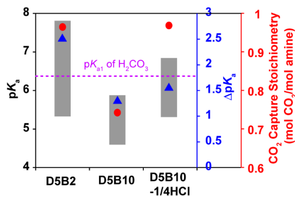
Fig. 2 pK_a values (left Y-axis) at 75 °C (bottom of bar) and 30 °C (top of bar), and \Delta pK_a values (blue right Y-axis, blue triangle) between 75 °C and 30 °C of D5B2 , D5B10 , and D5B10-1/4HCl , reversible CO 2 capture stoichiometries (red right Y-axis, red dot) of GP films in the temperature range 30–75 °C.
