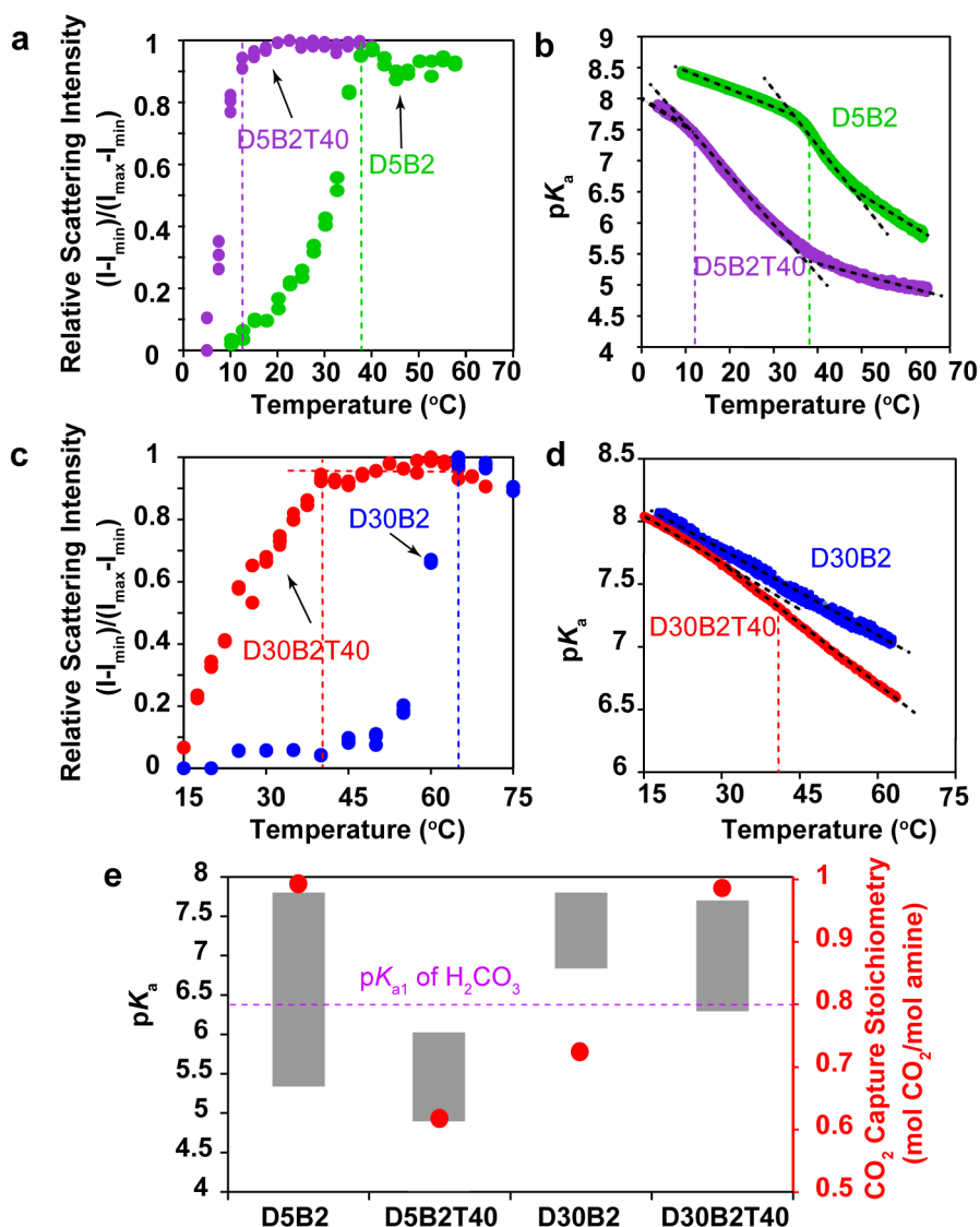
Fig. 3 (a) Relative scattering intensity as a function of temperature for D5B2 (green) and D5B2T40 (purple). (b) pK_a shift of D5B2 (green) and D5B2T40 (purple) during the heating process. (c) Relative scattering intensity as a function of temperature for D30B2 (blue) and D30B2T40 (red). (d) pK_a shift of D30B2 (blue) and D30B2T40 (red) during heating process. (e) pK_a values (left Y-axis) at 75 °C (bottom of bar) and 30 °C (top of bar) of the GPs, and reversible \text{CO}_2 capture stoichiometries (right Y-axis, red dot) of the GP films in the temperature range 30-75 °C.
