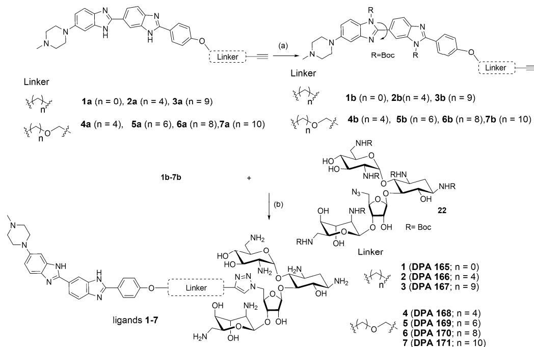
Scheme 2. (a) NaH, THF, (Boc) 2 O, rt, ~51-87 % overall yield (b) (i) CuSO 4 , sodium ascorbate, H 2 O, C 2 H 5 OH, rt, 24-30h (ii) trifluoroacetic acid, dichloromethane, rt, 3h (29-48 % yield for steps i and ii).
