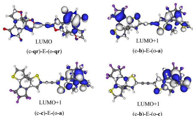
Fig. 7 Photocchromic virtual orbitals for the asymmetric dimers.
