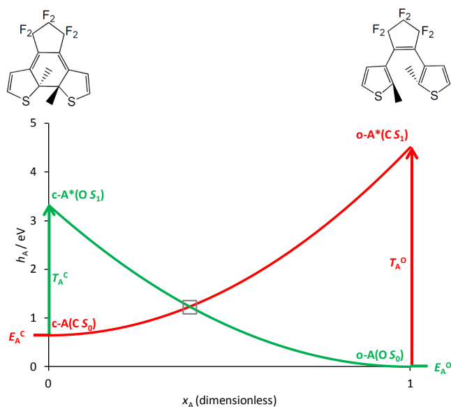
Fig. 2 Simplified correlation diagram for a single DAE unit A (red: state C; green: state O). x_A is the dimensionless reaction coordinate linking the open ( x_A=1 , rhs on the Figure) and closed ( x_A=0 , lhs on the Figure) isomers, h_A defines the relative energies (in eV). The energy parameters, corresponding to an isolated DAE displayed on top of the Figure, have been taken in Ref. 33.
