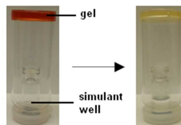
Figure 9 Experimental set up for testing the effects of DCP vapours on an organogel; Left) experimental setup without the presence of DCP in the simulant well; Right) effects of DCP addition to the simulant well.
