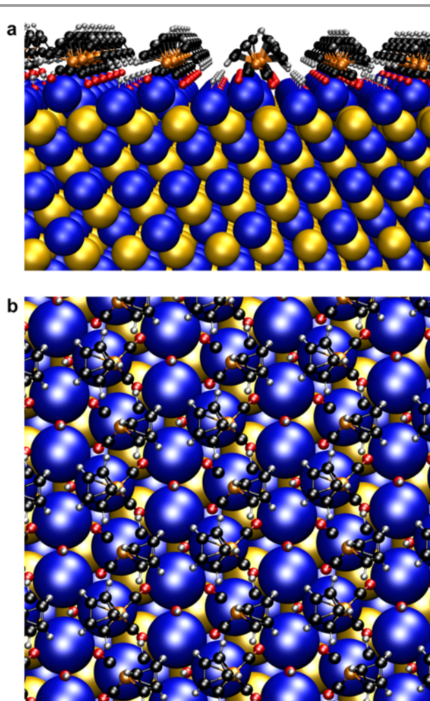
Fig. 7. Surface atomic structure of Fp beacons on the {111} face of PbSe. (a) Side-on view. (b) Top-down view. Following the work of Zhrebetskyy et al., one molar equivalent of -OH ligands relative to surface Pb(II) and Fp were used for charge balance 55 .
