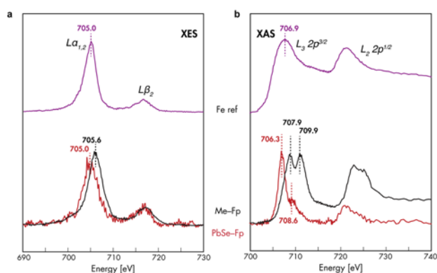
Fig. 3 Fe XES and XAS analysis of bonding in PbSe-Fp. (a) Fe L -edge XES and (b) Fe L -edge XAS spectra for PbSe-Fp (red), with related compound Me-Fp (black), and Fe reference standard (purple) shown for comparison. Fe reference spectra have been vertically offset for comparison.
