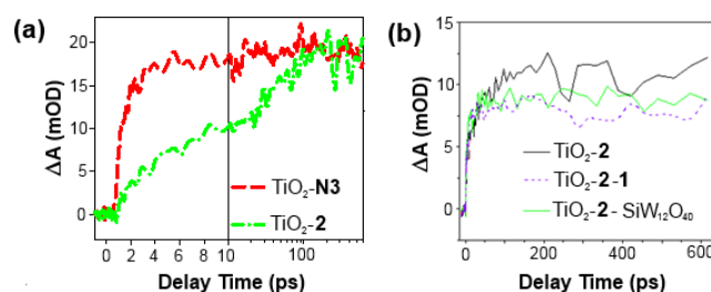
Fig. 4 Mid-IR comparison of the kinetics of electron injection in (a) \text{TiO}_2 - 2 and \text{TiO}_2 - N3 , and; (b) \text{TiO}_2 - 2-1 and \text{TiO}_2 - 2-SiW 12 O 40 . Data have been scaled to the absorbance of the supporting dyad film.
