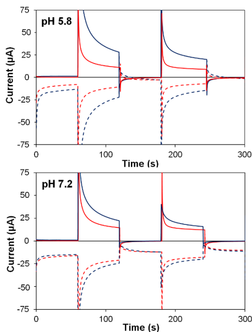
Fig. 7 Photoelectrochemical generator-collector measurements (chronoamperometry) of TiO 2 - 2 (red) and TiO 2 - 2Na 2 -1 (dark blue) at pH 5.8 and pH 7.2. Solid lines are the photoanode current; dashed lines, collector current; collector efficiency ca. 60%. Applied bias 0 mV vs Ag/AgCl, illuminated with a 455 nm LED (33 mW cm -2 ). Photocurrent densities are reported in Table 4.
