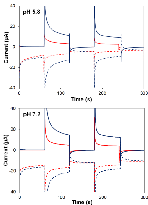
Fig. 6 Photoelectrochemical generator-collector measurements (chronoamperometry) of TiO 2 - P2 (red) and TiO 2 - 2 (dark blue) at pH 5.8 and pH 7.2. Solid lines are the photoanode current; dashed lines, collector current; collector efficiency ca. 60%. Applied bias 0 mV vs Ag/AgCl, illuminated with a 455 nm LED (33 mW cm -2 ). Photocurrent densities are reported in Table 4.
