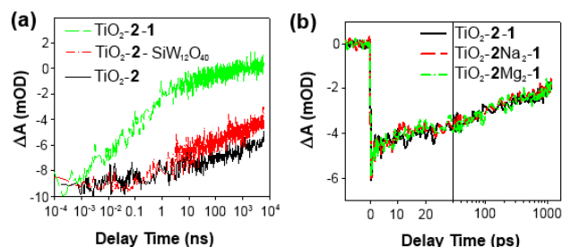
Fig. 5 (a) Ground state bleach recovery kinetics of TiO 2 - 2 (black), TiO 2 - 2-SiW 12 O 40 (red) and TiO 2 - 2-1 . (b) Ground state bleach recovery kinetics of TiO 2 - 2-1 (black), TiO 2 - 2-Na 2 -1 (red) and TiO 2 - 2-Mg 2 -1 (green).
