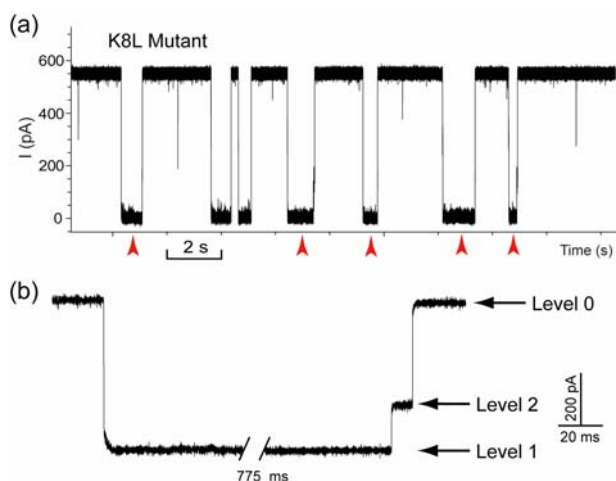
Fig. 4 Translocation of DNA1-Fc-CB[7] through engineered \alpha HL mutant K8L. (a) Representative current trace of the translocation of DNA1-Fc-CB[7] through mutant K8L. Red arrows indicate the multi-level current events. (b) Expanded view of a multi-level signature event. Traces were recorded in 3 M KCl buffered with 10 mM Tris, pH 8.0. DNA1-Fc (final concentration 0.25 \mu M) were incubated with CB[7] (final concentration 50 \mu M) at room temperature for 2 hours before measurement. The transmembrane potential was held at +200 mV.
