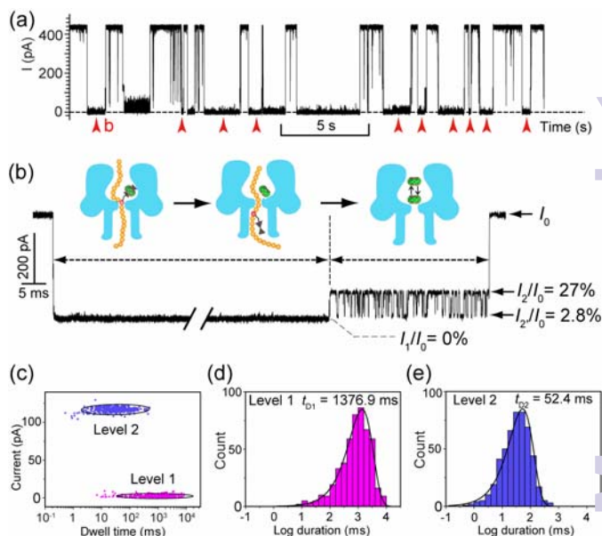
Fig. 3 Translocation of a hybrid of DNA1-Fc \subset CB[7] through \alpha HL. (a) A representative current trace of the translocation of DNA1-Fc \subset CB[7] (final concentration 0.25 \mu M) through \alpha HL. Data were acquired in the buffer of 3 M KCl and 10 mM Tris, pH 8.0, with the transmembrane potential held at +160 mV. Red arrows indicate the multi-level current events. (b) A typical multi-level signature event generated by the DNA1-Fc \subset CB[7] translocation (marked in (a)). Diagrams above the trace show the molecular mechanism of hybrid dissociation and translocation. Level 0: the open pore current level. Level 1: trapping of DNA1-Fc \subset CB[7] in the pore, dissociation of the DNA1-Fc \subset CB[7] and translocation of the DNA1-Fc through the pore. Level 2 and 2': oscillation of CB[7] in the cis vestibule of \alpha HL. (c) Scatter plots showing current blockage versus event durations of Level 1 and Level 2 in the signature events. (d) Dwell-time histogram for Level 1. The solid line in the histogram is a single exponential fit to the data. For Level 1, the mean duration t_{D1} = 1376.9 ms. (e) Dwell-time histogram for Level 2. The solid line in the histogram is a single exponential fit to the data. For Level 2, the mean duration t_{D2} = 52.4 ms. The sequence of DNA1: 5'-AAAAAAAAAA(5mC)AAAAAAAAA-3'.
