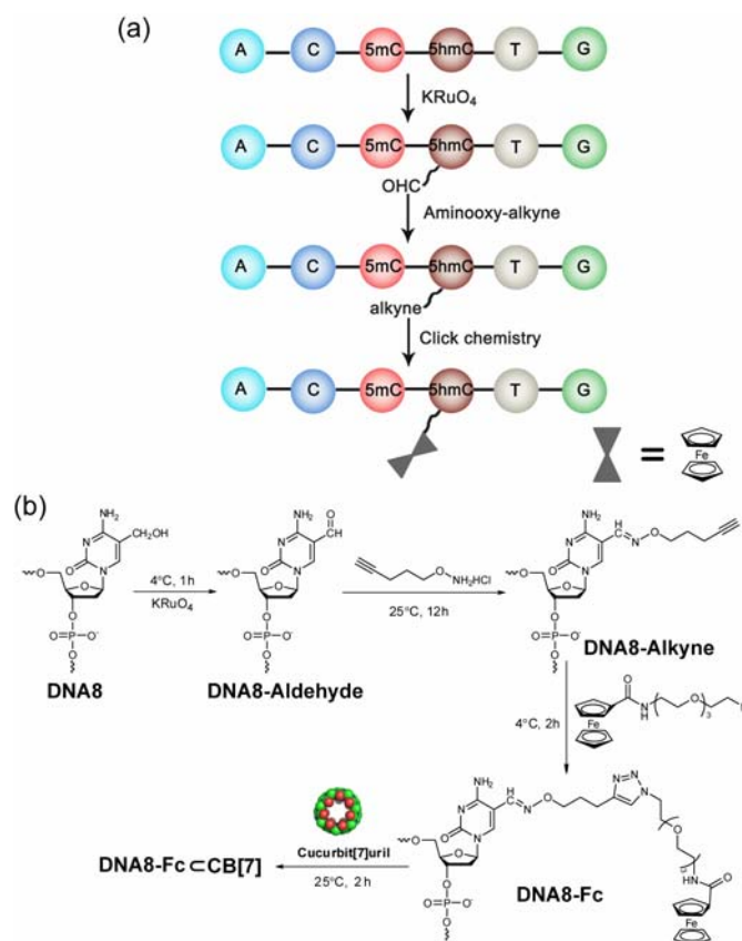
Fig. 2 Selective modifications of 5hmC-containing DNA. (a) Selective modification steps of 5hmC-containing DNA8 to afford the covalent DNA8-Fc complex. (b) Chemical reactions of the modification of DNA8.
