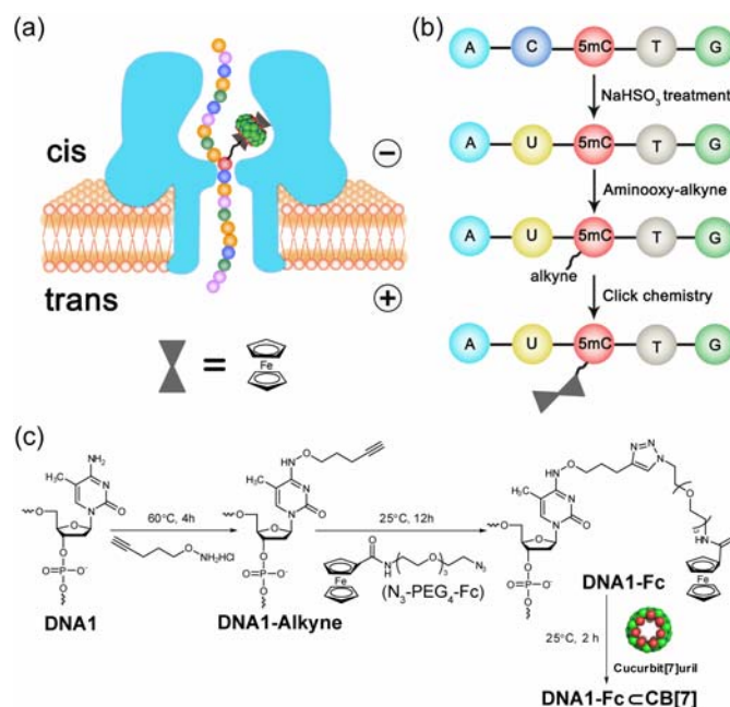
Fig. 1 Schematic illustration of the detection strategy and chemical labeling of 5mC-DNA. (a) Translocation of a 5mC/5hmC-containing DNA molecule modified with Fc-cCB[7] complex through \alpha HL nanopore. (b) Selective modification steps of 5mC-DNA to afford the covalent DNA-Fc complex. The aminoxy-alkyne is O -(pent-4-yn-1-yl)hydroxylamine. (c) Chemical reactions of the modifications of 5mC-DNA in (b).
