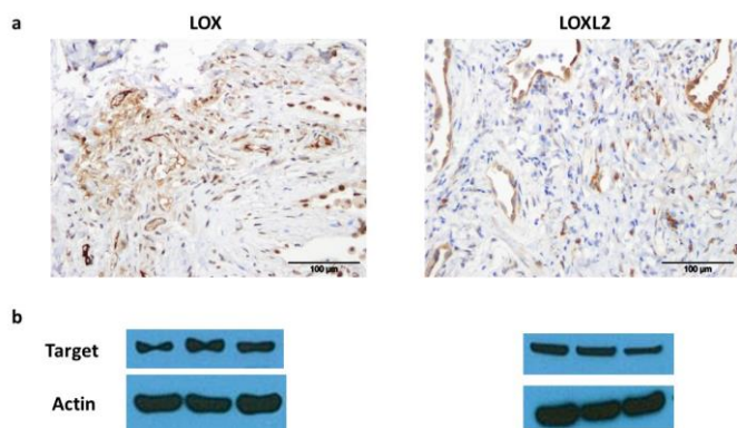
Fig. 1: LOX and LOXL2 are expressed in aged human lung tissue homogenates. (a). Immunohistochemical analysis and (b). western blot of LOX and LOXL2 expression in aged (55-81yr) human lung tissue. Strongest bands for LOX were at 50kDa, consistent with the glycosylated pro-lysyl oxidase, but mature 32kDa LOX was also present in several samples (ESI, Figure S1). Data representative of a minimum of 3 experimental replicates. Scale-bar = 100 \mu m.
