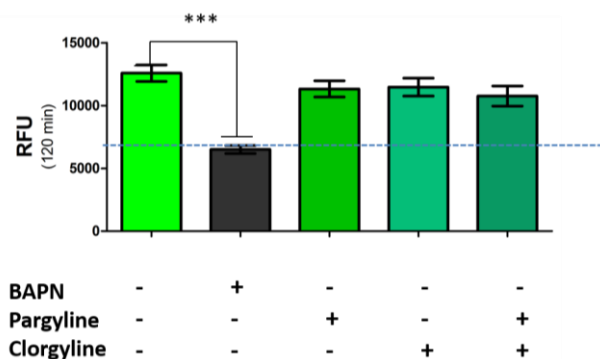
Fig. 3 oLOX is not activated by monoamine oxidases. Human
