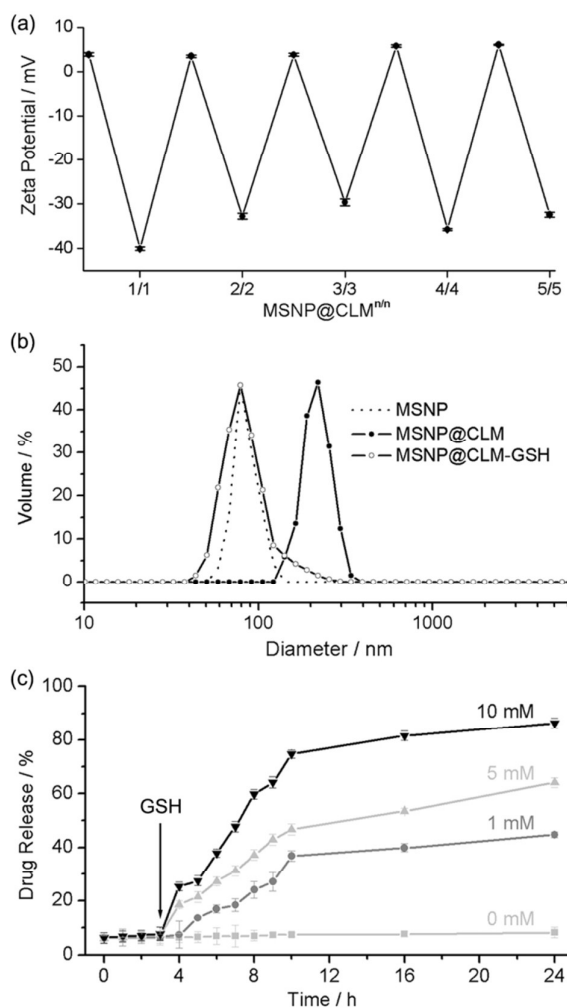
Fig. 4 (a) Zeta-potential values measured during multilayer preparation. (b) Hydrodynamic diameters of MSNPs, MSNP@CLM 5/5 , and MSNP@CLM 5/5 after GSH treatment. (c) Stimulus-triggered drug-release profiles with different GSH concentrations. GSH was added at 3 h.
