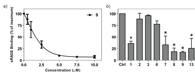
Fig. 6 a) Succinyl surfen ( 9 ) dose-dependently inhibits sRAGE binding to HS. b) sRAGE binding inhibitory activity of selected compounds at 10 μM. The values represent the means ± SD. *P < 0.0001 compared with a control in the absence of antagonist.
