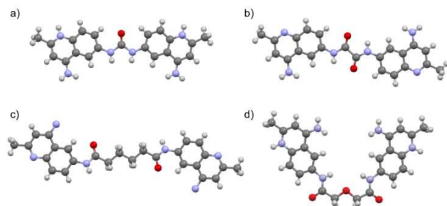
Fig. 3 X-ray crystal structures of a) surfen•2CF 3 COOH ( 1 ), b) oxalyl surfen ( 7 ), c) adipoyl surfen ( 11 ), and d) diglycolyl surfen•2HCl ( 13 ). Counterions and solvent molecules omitted for clarity (See SI for additional information).
