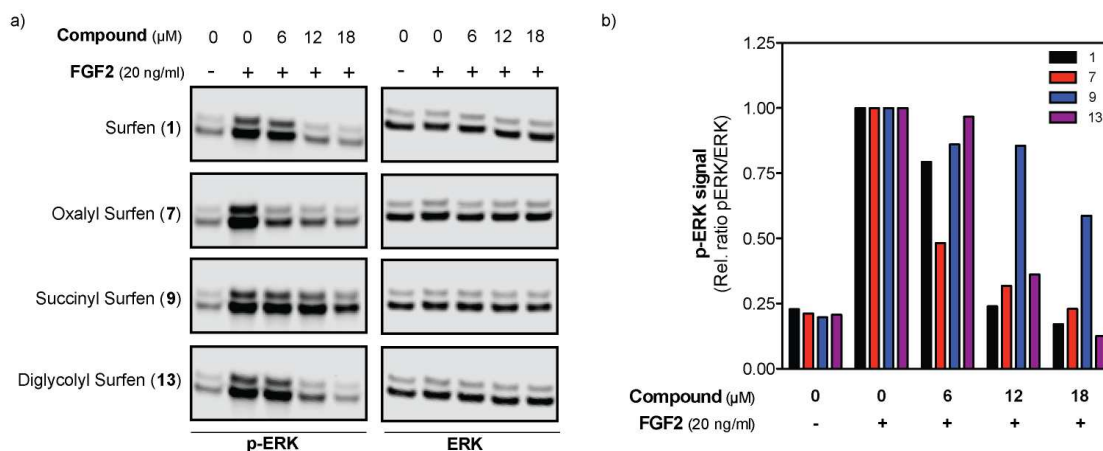
Fig. 5 Surfen and selected analogs inhibit FGF2-induced ERK phosphorylation. a) Western blot analysis of the inhibition of downstream FGF-2 induced ERK phosphorylation (p-ERK), b) band intensities were quantitated by densitometry and plotted as the ratio of p-ERK to ERK signal.
