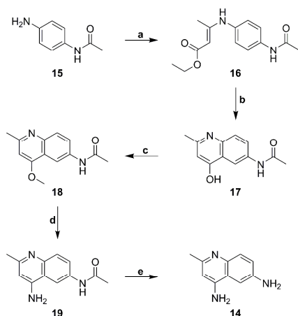
Scheme 1 Synthesis of 4,6-diamino-2-methylquinoline building block ( 14 ) (a) ethyl acetoacetate, MeOH, reflux, (b) Dowtherm A, 265°C, (c) dimethyl sulfate, toluene, 120°C, (d) ammonium acetate, 135°C, (e) 37% HCl, 90°C.
