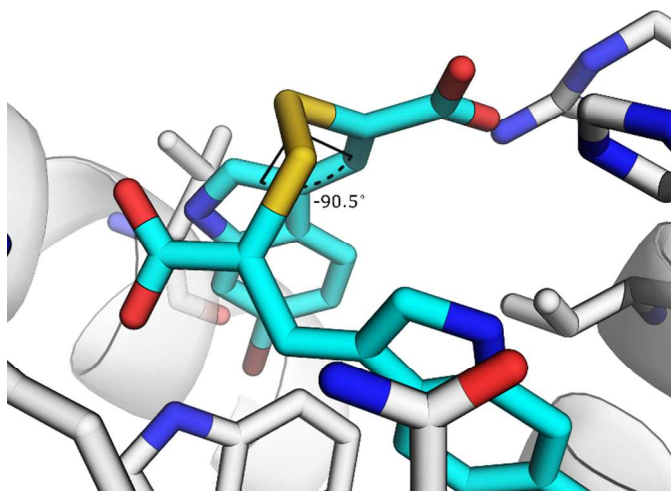
Fig. 5: Representation of 4 with a dihedral angle of -90.5° bound to chain A of PEF(S).
