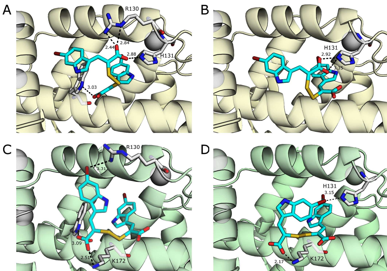
Fig. 3: Comparison of the two conformations 4 (cyan) bound to chain A (yellow) of the PEF(S) homodimer, (A) and (B) respectively, and chain B (green) of the homodimer, (C) and (D) respectively. Residues that form halogen bonds, hydrogen bonds and electrostatic interactions are highlighted and important bonds are indicated by dashed lines, distances are shown in Å (PDB 4WQ2 and 4WQ3).
