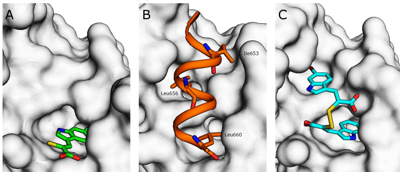
Fig. 2: (A) Surface representation of chain A of PEF(S) bound to 3 in the hydrophobic pocket that binds Leu 660 (PDB 4WQ2). (B) Inhibitory region C of the CAST domain IV bound to PEF(S); Ile 653, Leu 656 and Leu 660 are highlighted (PDB:3BOW). 23 (C) 4 bound to chain A of PEF(S); a single binding mode of 4 is represented (PDB 4WQ3).
