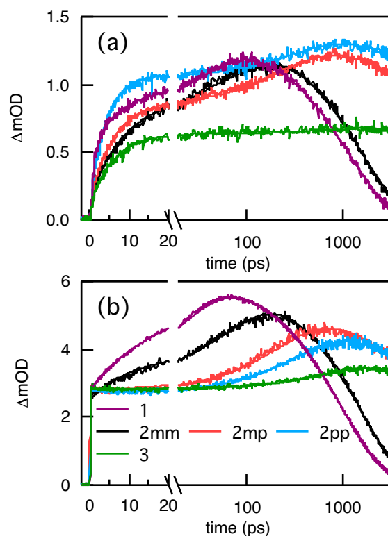
Fig. 6 Kinetic traces of \Delta OD at 710 nm (main absorption band of PDI^{-\cdot} ) upon pulsed laser excitation at 350 nm (a) and 527 nm (b). The thick solid lines are the fits to the data obtained from global and target analysis.
